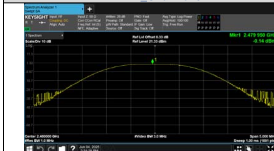
Peak Output Power BLE 1M_Channel 39
