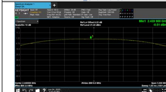
Peak Output Power BLE 2M_Channel 19
