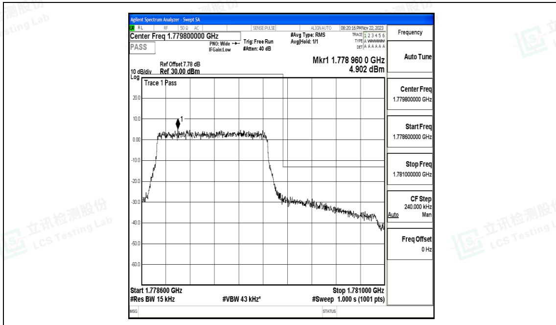
Band66_1.4MHz_QPSK_132665_6RB#0
