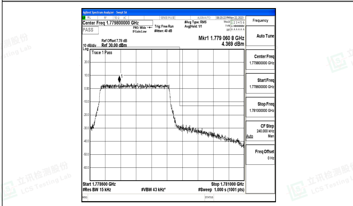
Band66_1.4MHz_16QAM_132665_6RB#0
