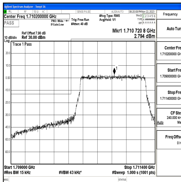
Band66_1.4MHz_16QAM_131979_6RB#0
