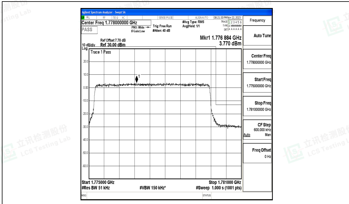
Band66_5MHz_QPSK_132647_25RB#0
