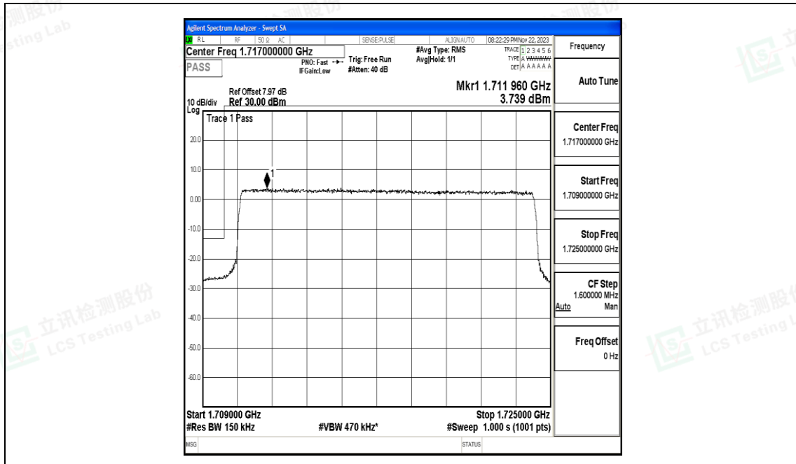
Band66_15MHz_QPSK_132047_75RB#0
