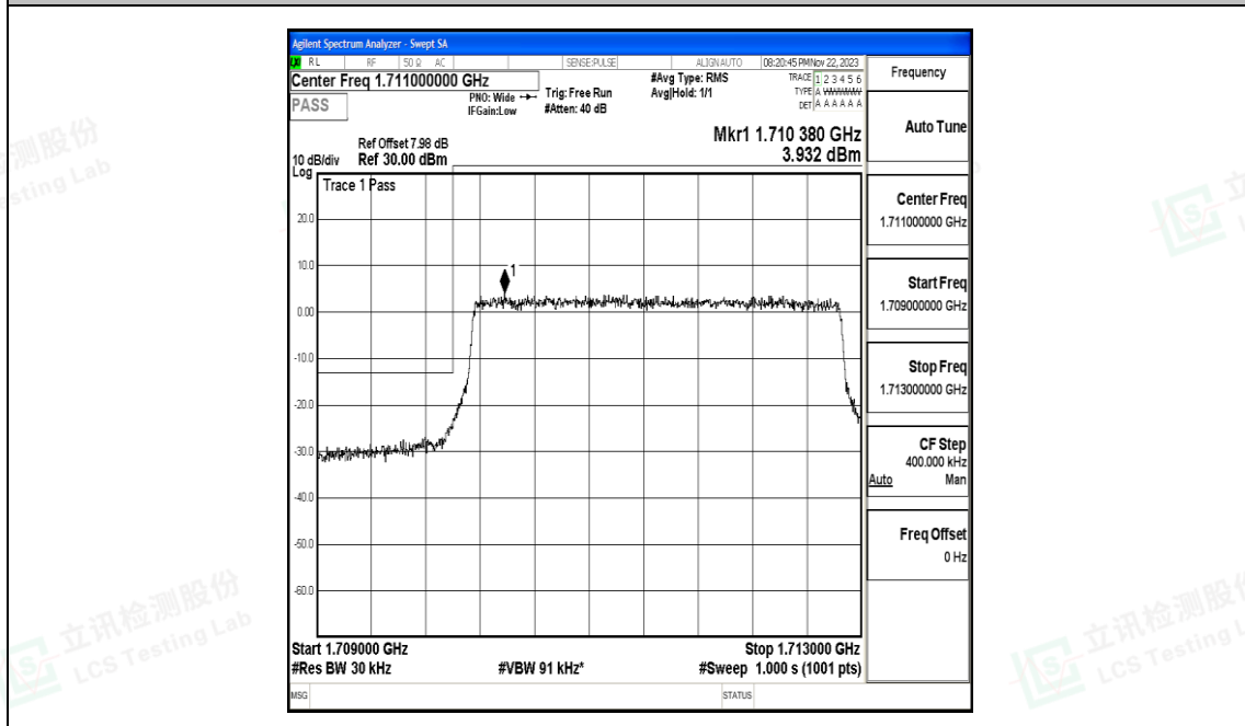
Band66_3MHz_16QAM_131987_15RB#0
