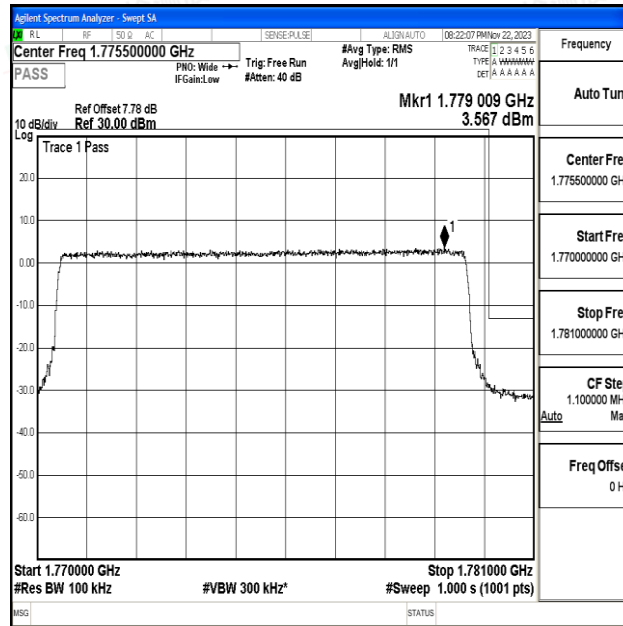
Band66_10MHz_QPSK_132622_50RB#0
