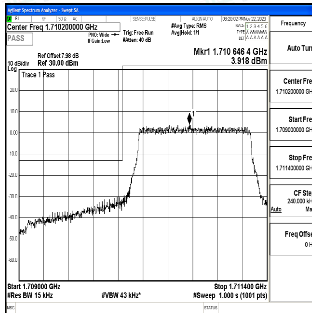
Band66_1.4MHz_QPSK_131979_6RB#0
