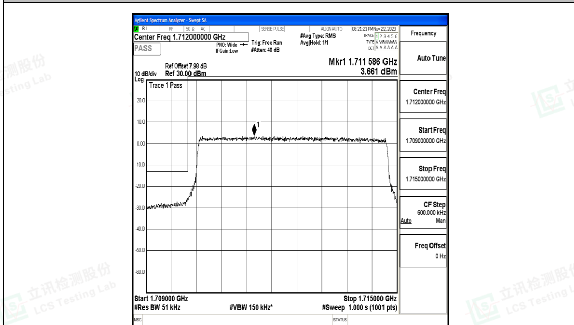
Band66_5MHz_16QAM_131997_25RB#0
