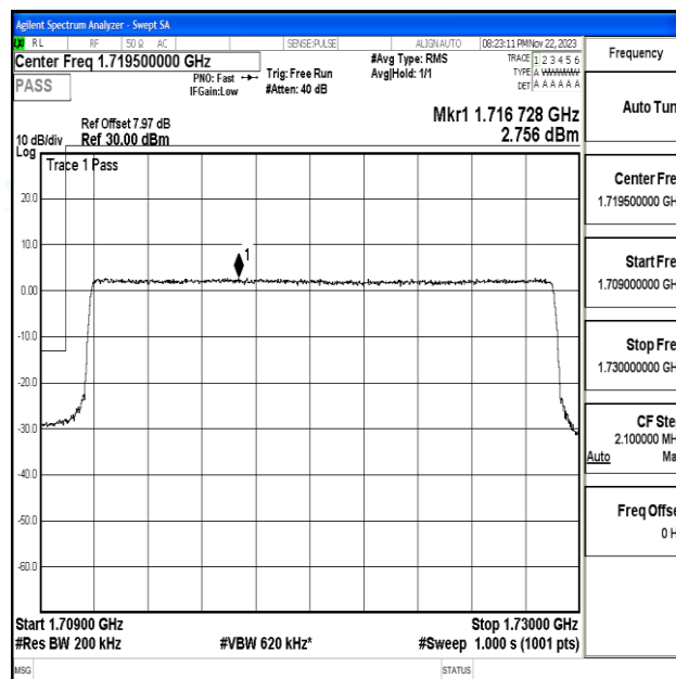
Band66_20MHz_16QAM_132072_100RB#0
