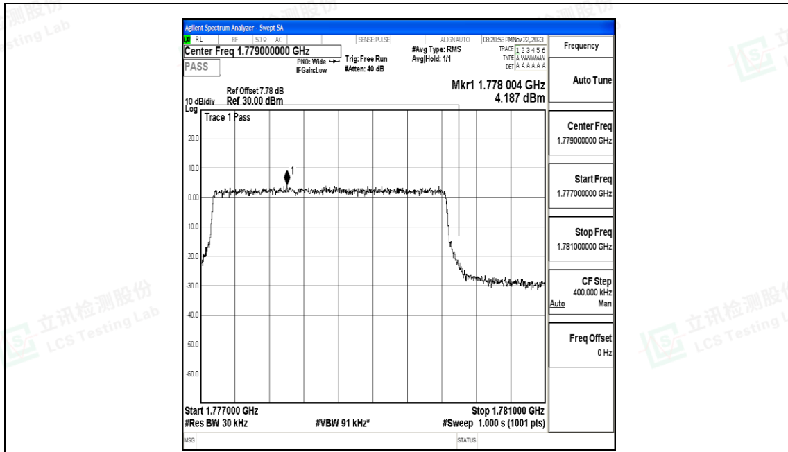
Band66_3MHz_QPSK_132657_15RB#0
