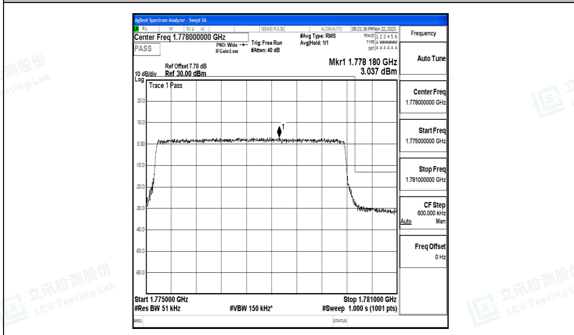
Band66_5MHz_16QAM_132647_25RB#0
