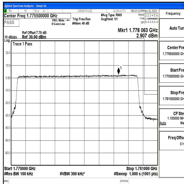
Band66_10MHz_16QAM_132622_50RB#0
