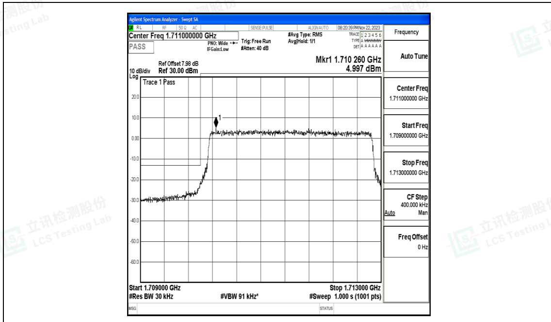
Band66_3MHz_QPSK_131987_15RB#0
