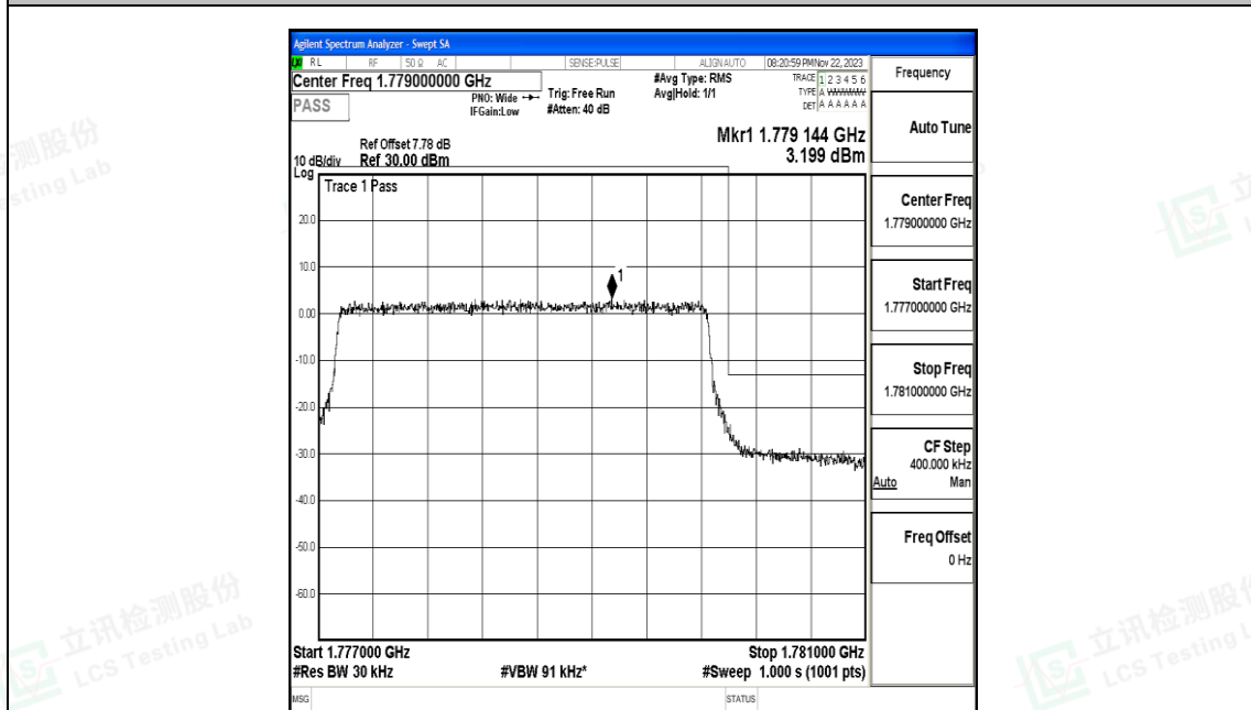
Band66_3MHz_16QAM_132657_15RB#0
