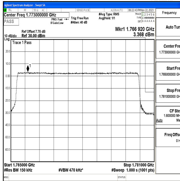
Band66_15MHz_QPSK_132597_75RB#0
