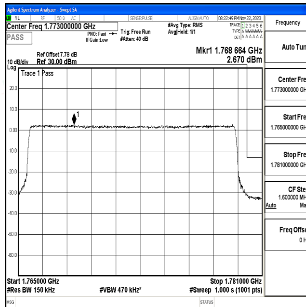
Band66_15MHz_16QAM_132597_75RB#0
