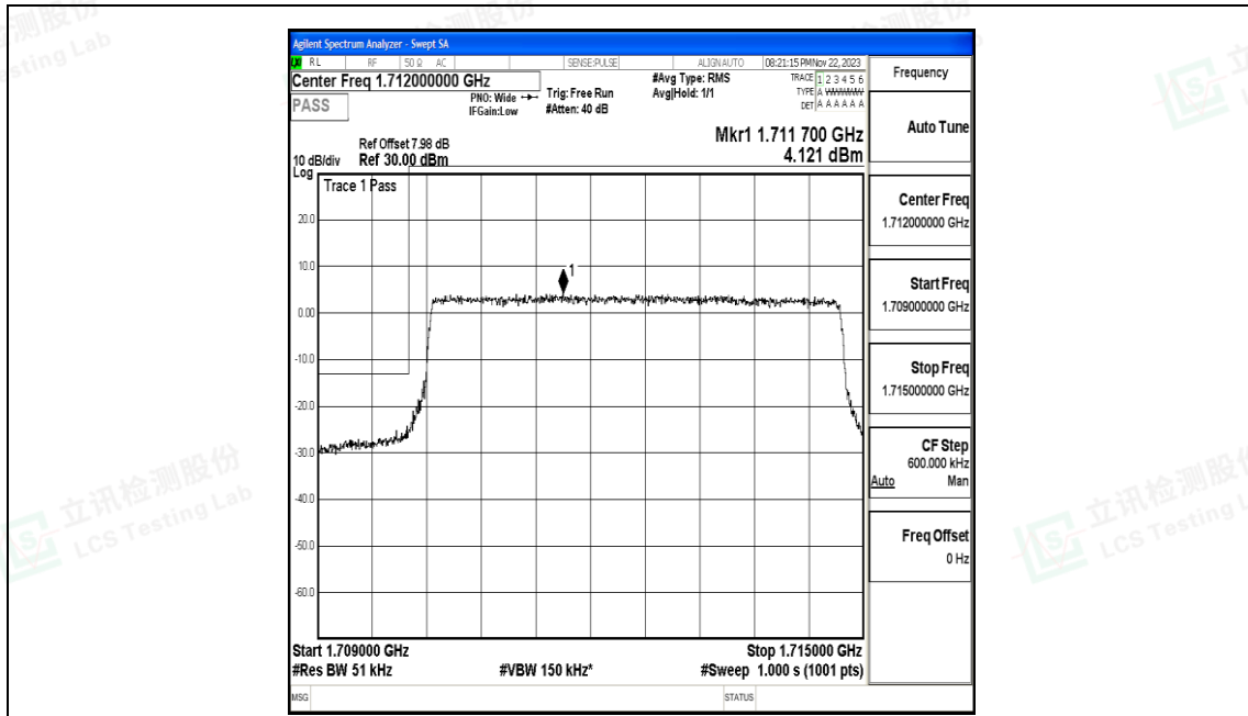
Band66_5MHz_QPSK_131997_25RB#0
