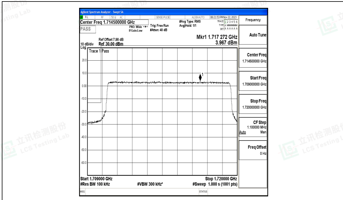
Band66_10MHz_QPSK_132022_50RB#0
