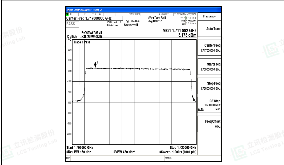
Band66_15MHz_16QAM_132047_75RB#0
