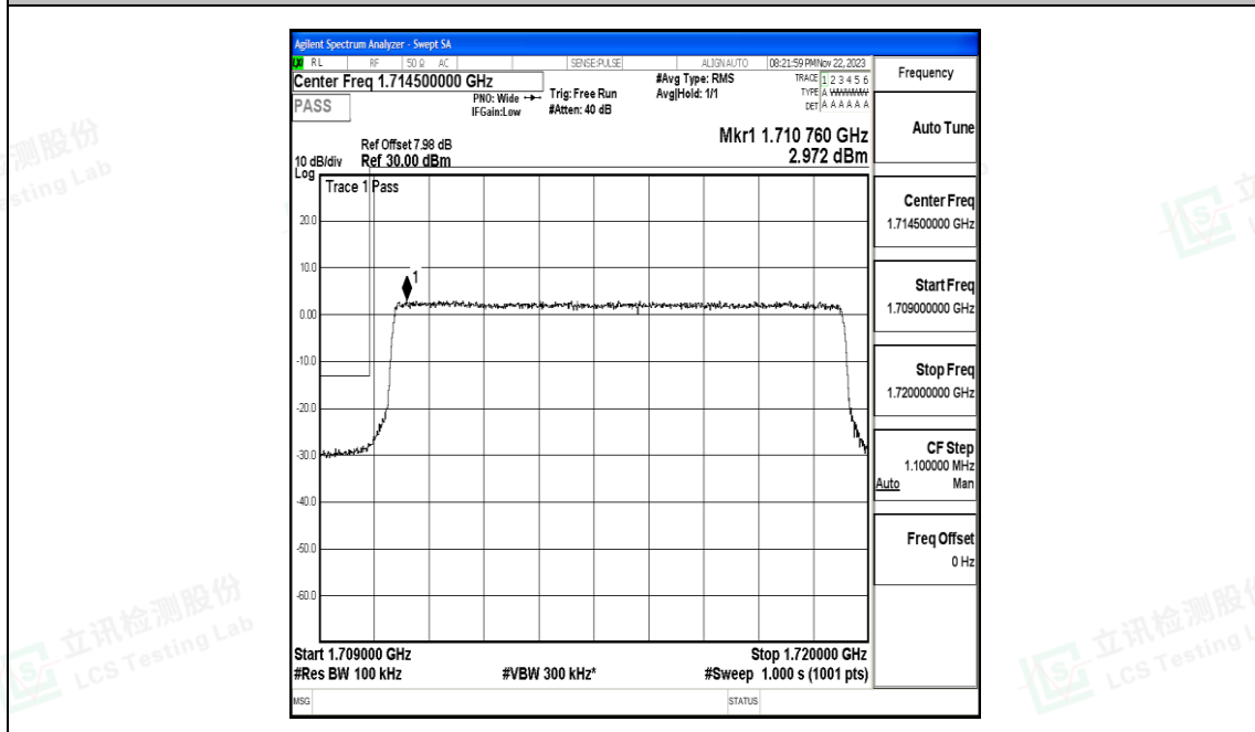
Band66_10MHz_16QAM_132022_50RB#0
