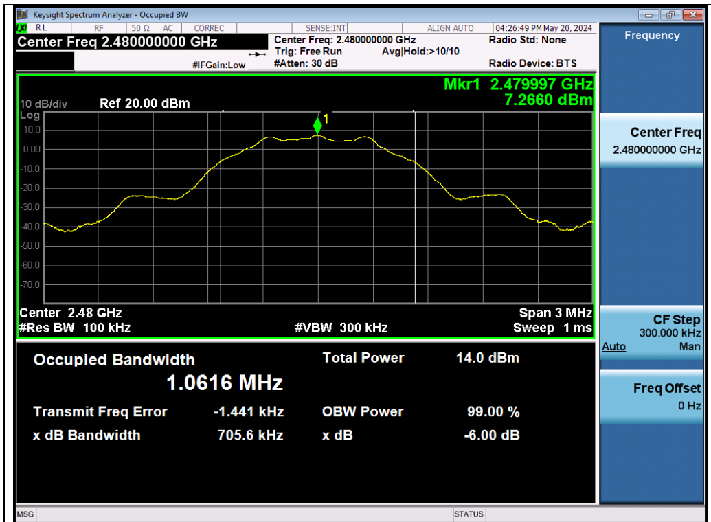
Test_Graph_LE1M_ANT1_2480_1Mbps_DTBSW
