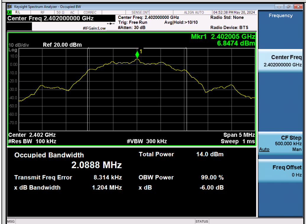
Test_Graph_LE2M_ANT1_2402_2Mbps_DTBSW
