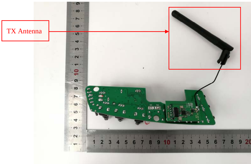
EUT – Transmitter PCB Top View(TF-41)
