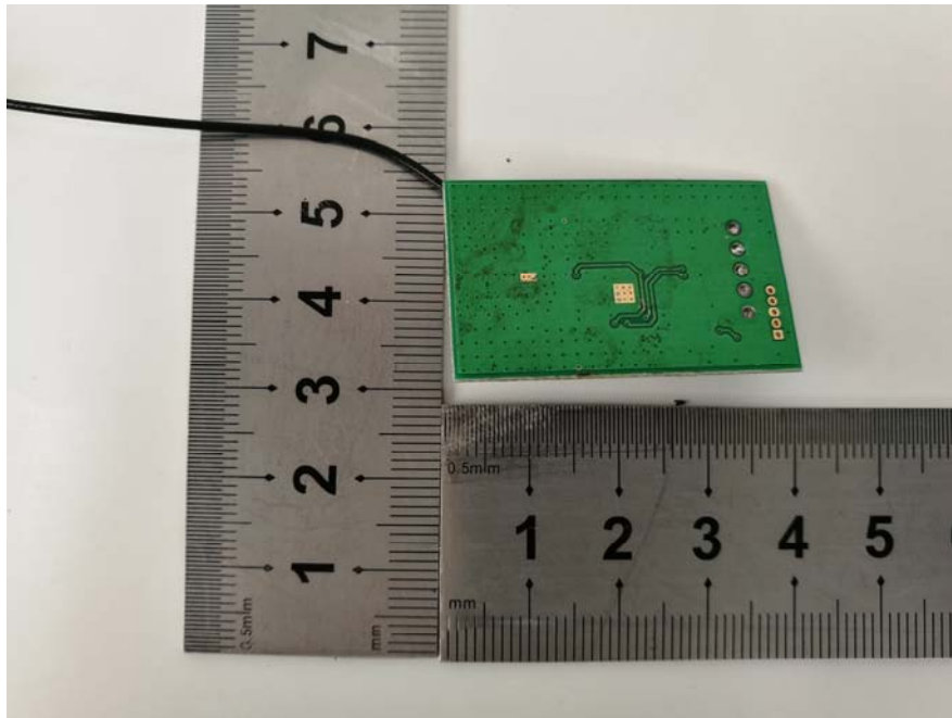
EUT – Transmitter Module Bottom View(TF-41)
