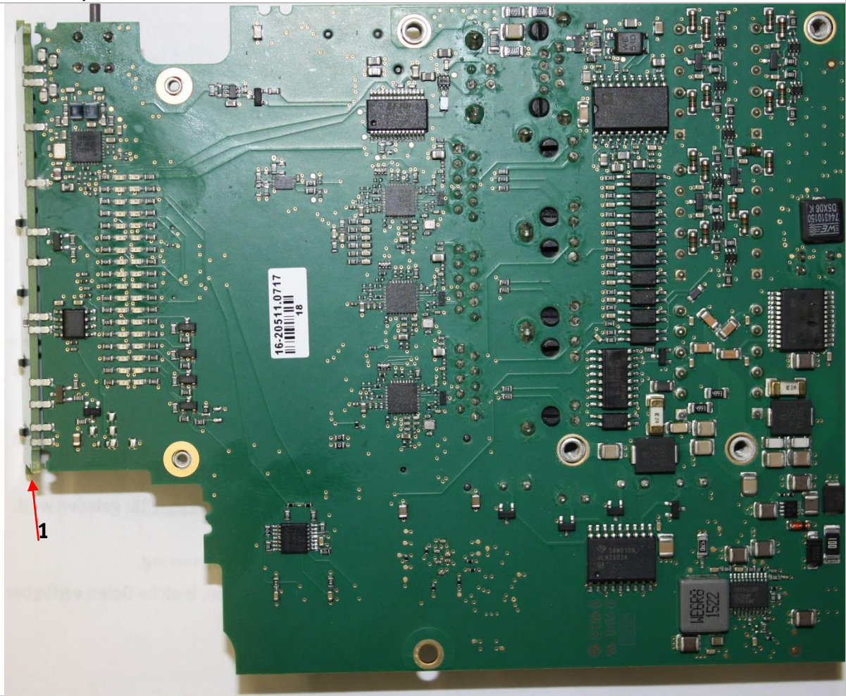
1 Header PCB with NFC and RFID antenna
