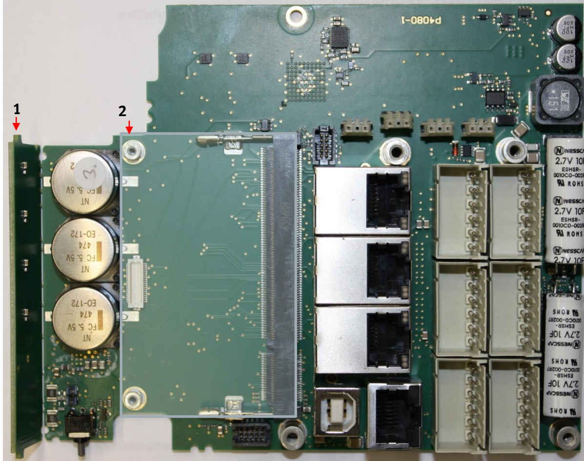
1 Header PCB with NFC and RFID antenna 2 Sockets / Place for SoC-Module
