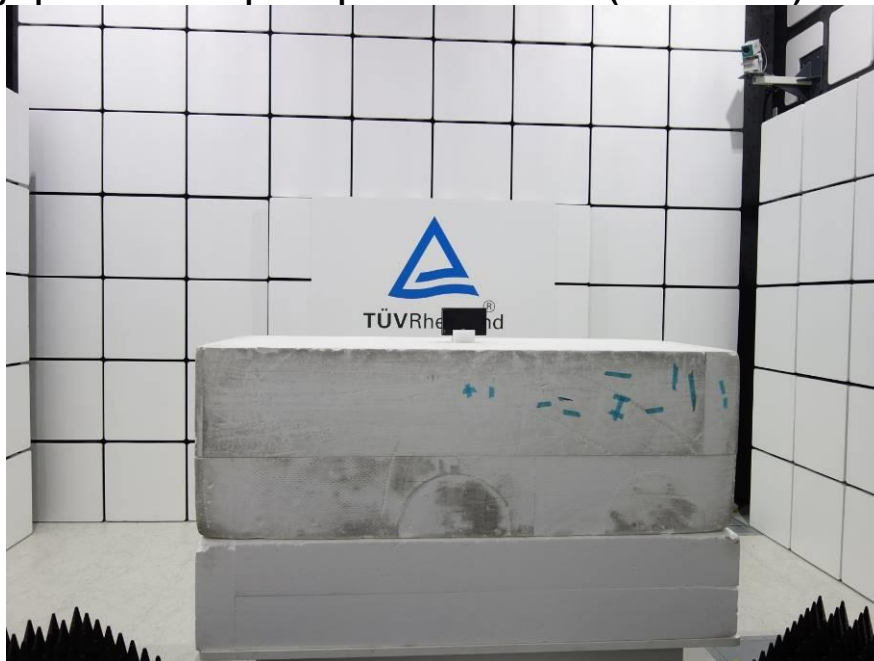
Photograph 4: Test Setup for Spurious Emissions (Front View 1)
