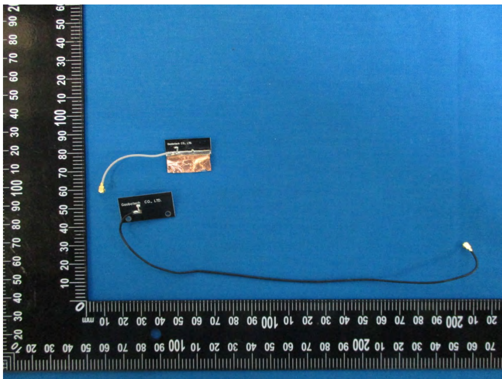
Bluetooth and Wifi Antenna Antenna View
