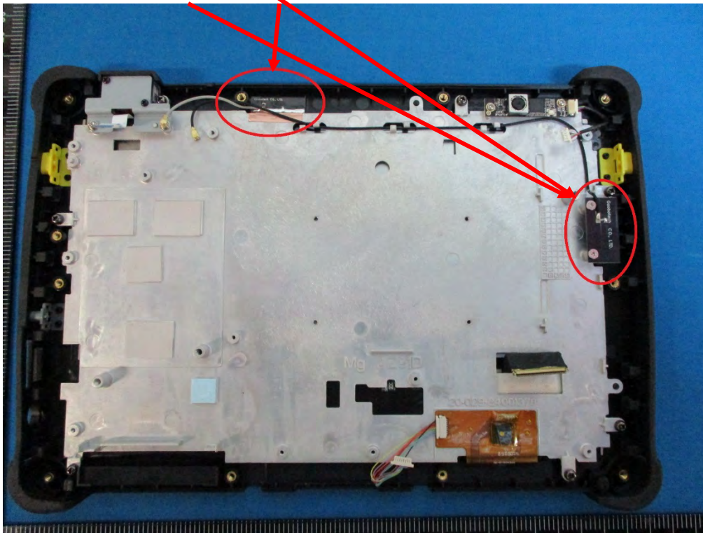
Bluetooth and Wifi Antenna – Location View
