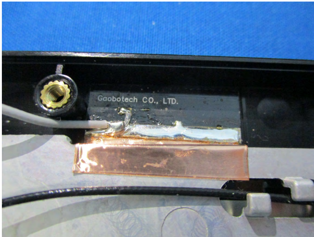
Wifi Antenna(Chain 1) View
