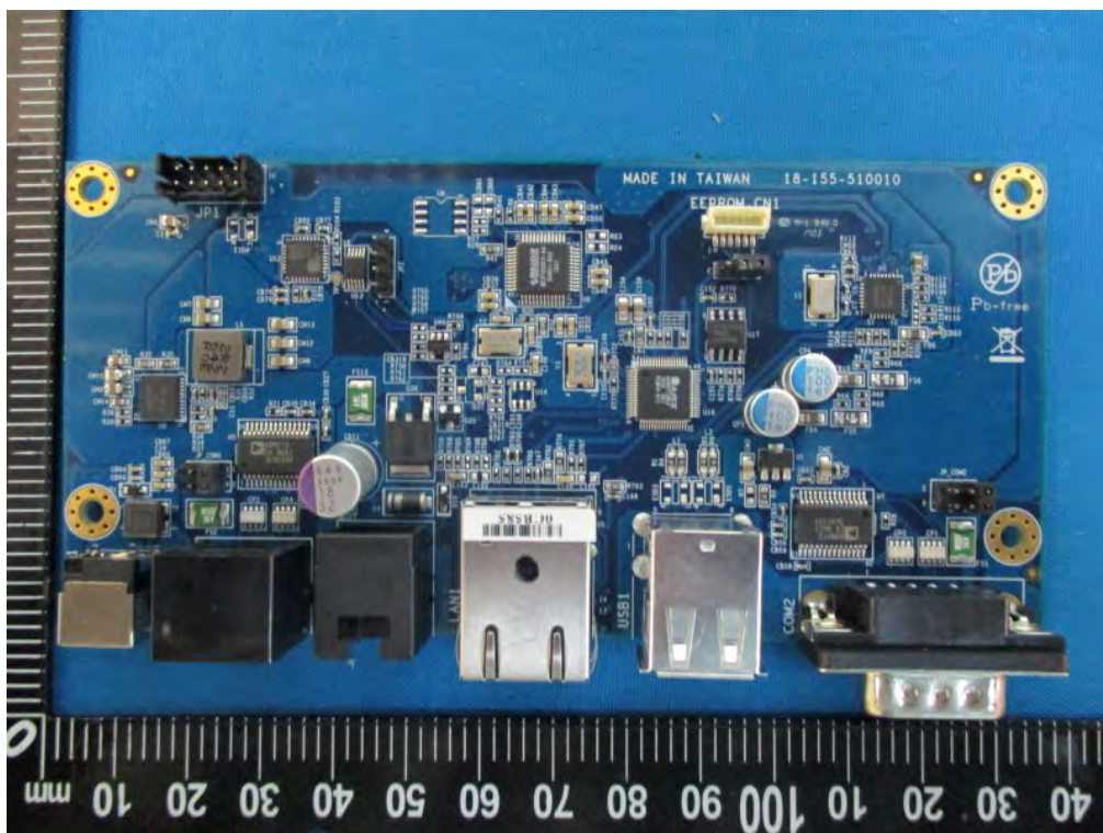
Black Cradle - Main Board Top View
