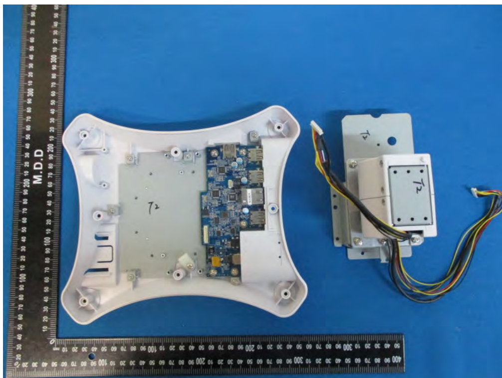
White Cradle - Uncover View
