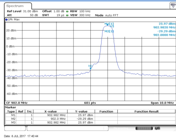
LOW CHANNEL, Band Edge
