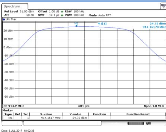
High CHANNEL, Carrier level
