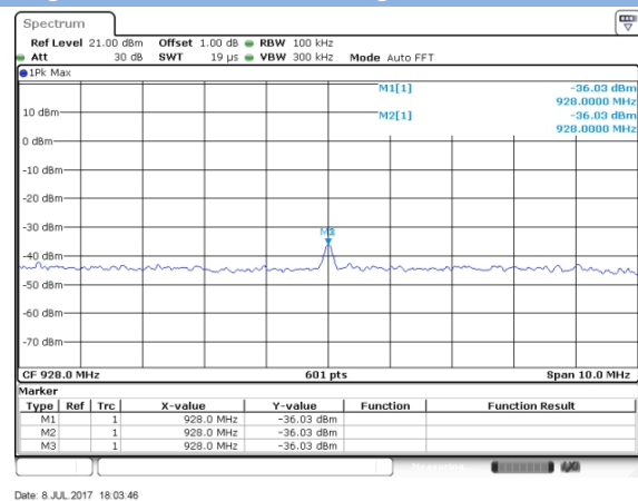
High CHANNEL, Band Edge
