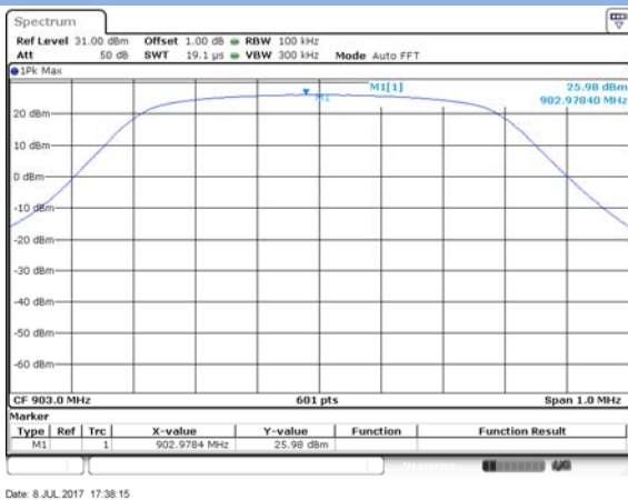
LOW CHANNEL, Carrier level
