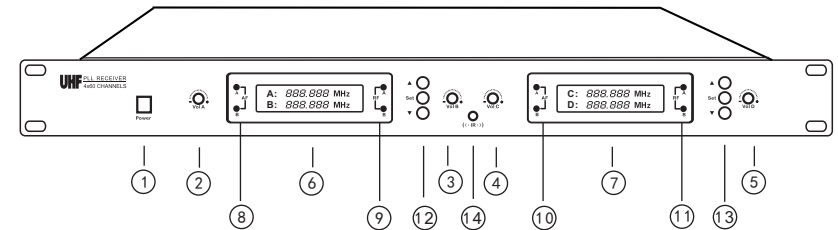
Front panel of 4 channel receiver
