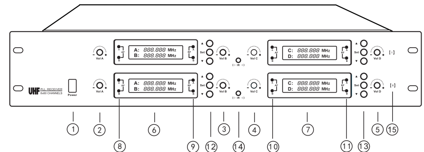
Front panel of 8 channel receiver
