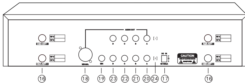
Rear panel of 8 channel receiver
