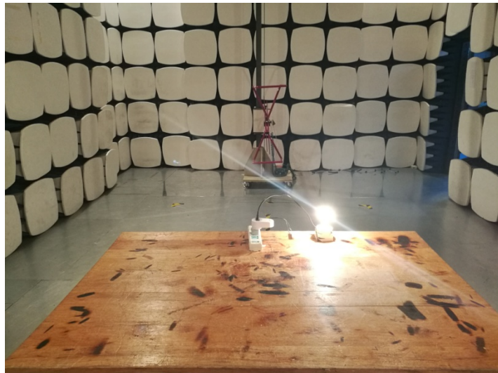
Radiated Emission
