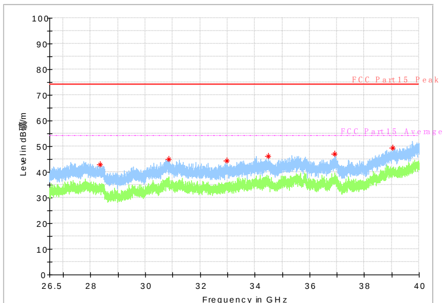
Fig. 61 Radiated emission: 802.11n, (802.11n-HT40, Ch151, 26.5 GHz - 40 GHz)
