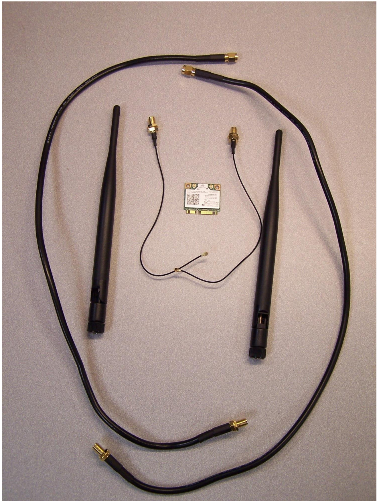
Radio with internal coax cables (small); external coax cables (large); antennas
