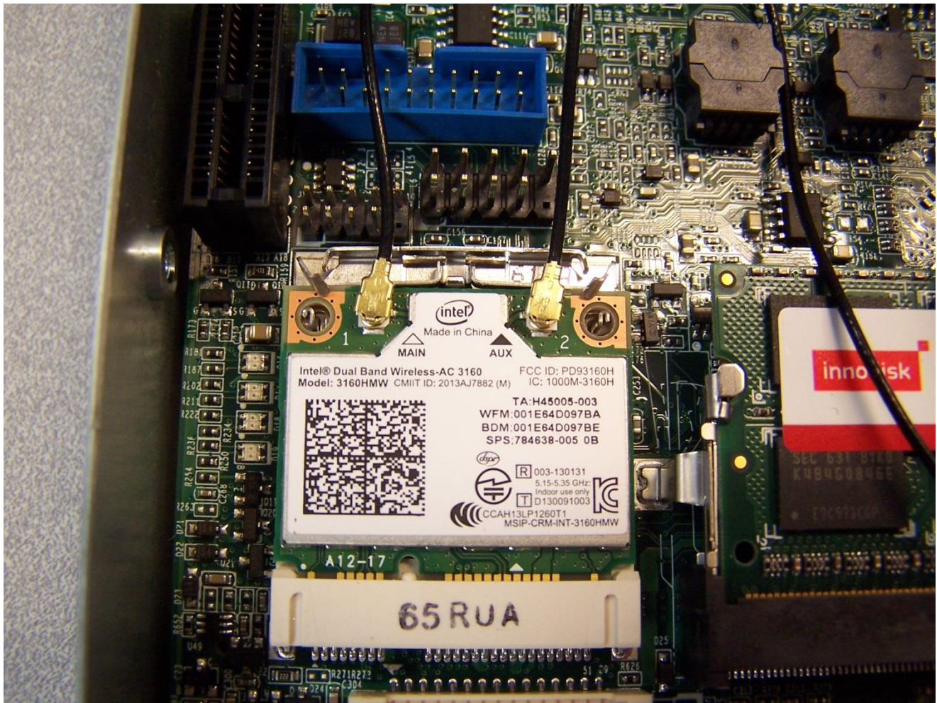
Enlarged view of Radio installed in WiSP
