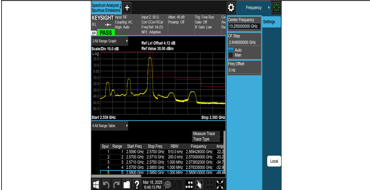
Band7-10MHz-16QAM-20800-1RB#0-PASS
