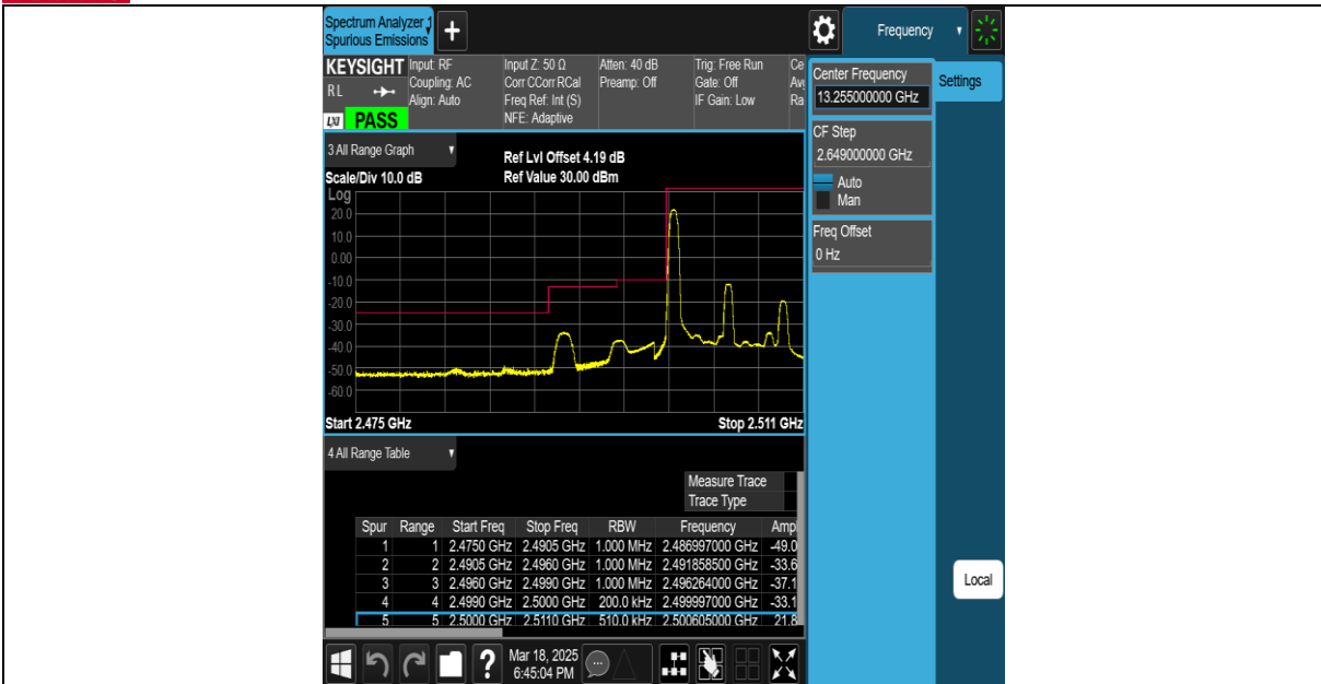
Band7-10MHz-QPSK-20800-50RB#0-PASS
