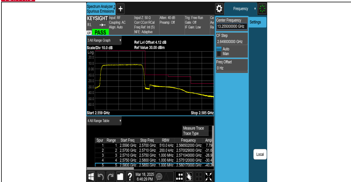
Band7-10MHz-QPSK-21400-1RB#49-PASS
