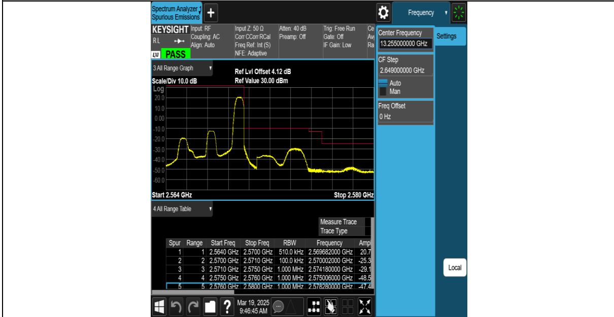
Band7-10MHz-QPSK-20800-1RB#0-PASS
