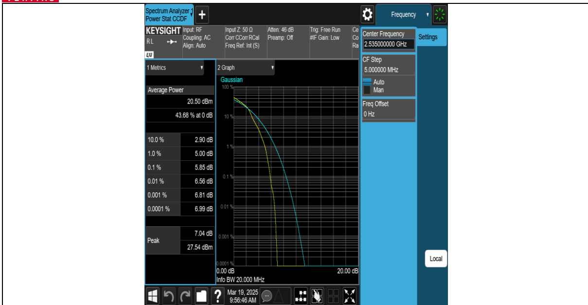
Band7-20MHz-16QAM-21100-27RB#0-PASS
