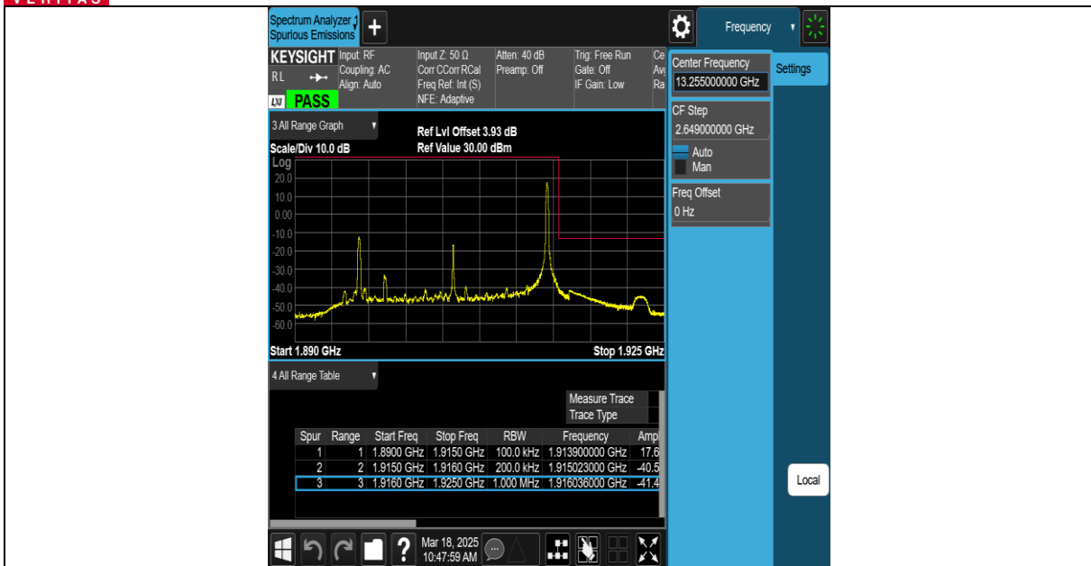
Band25-20MHz-16QAM-26140-1RB#0-PASS
