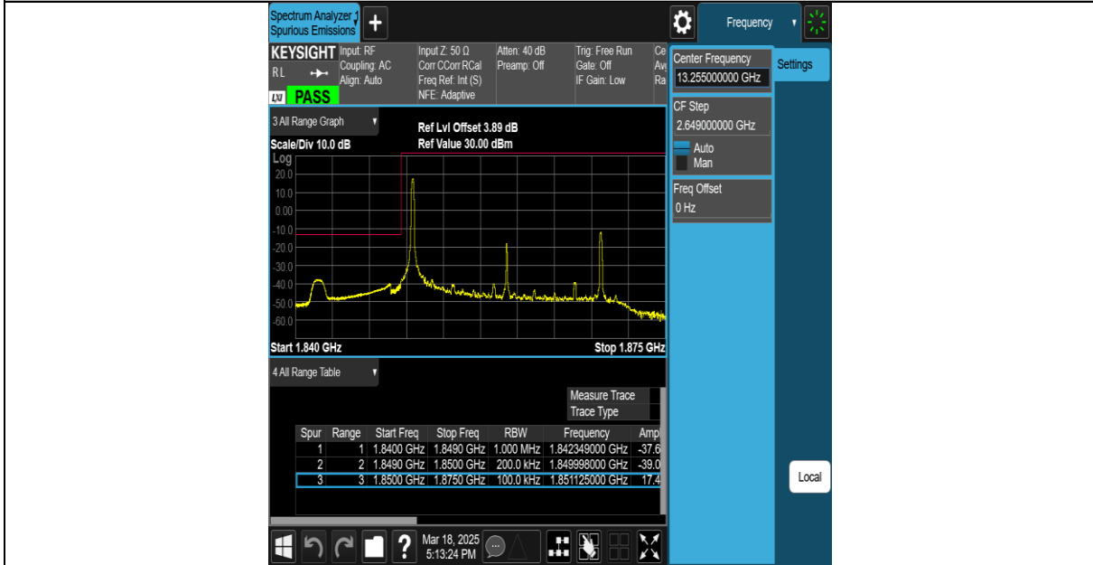
Band25-20MHz-16QAM-26140-27RB#0-PASS
