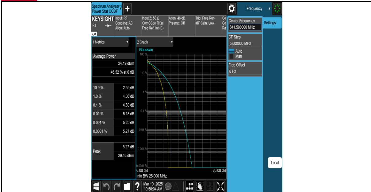
26(824-849)-15MHz-QPSK-26965-75RB#0-PASS
