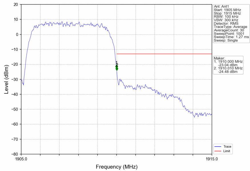
Band2_RMC_HCH_1907.6MHz_12.2kbps RMC_NTNV
