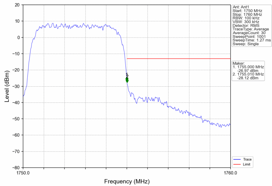
Band4_RMC_HCH_1752.6MHz_12.2kbps RMC_NTNV
