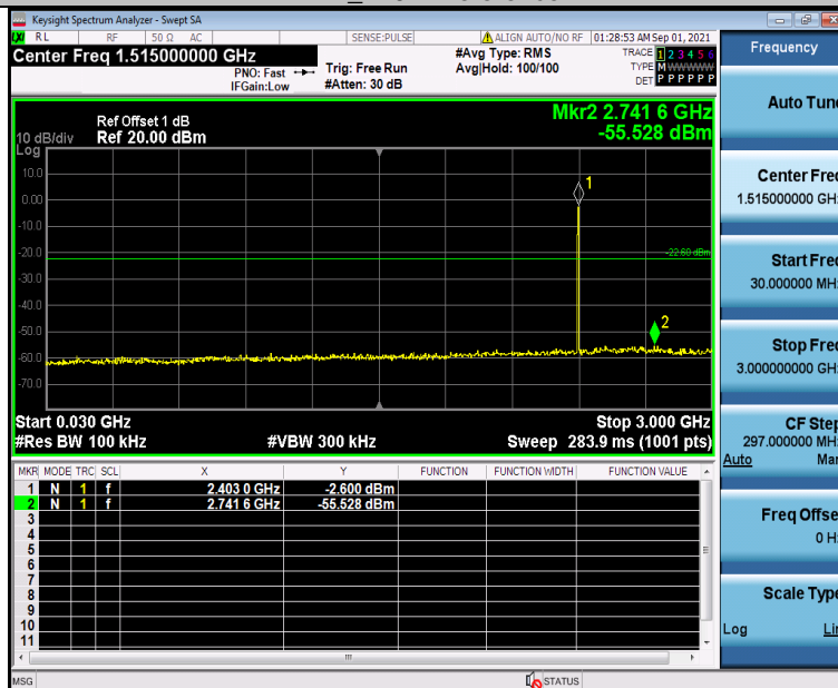
BLE_2402_30-3000
