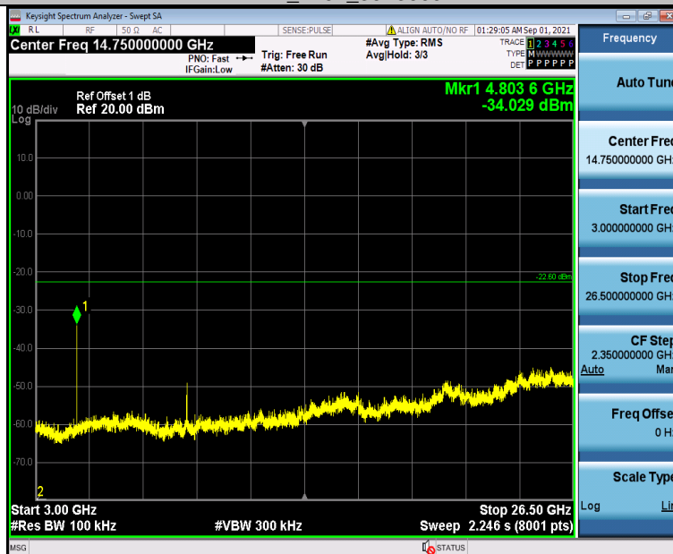
BLE_2402_3000-26500
