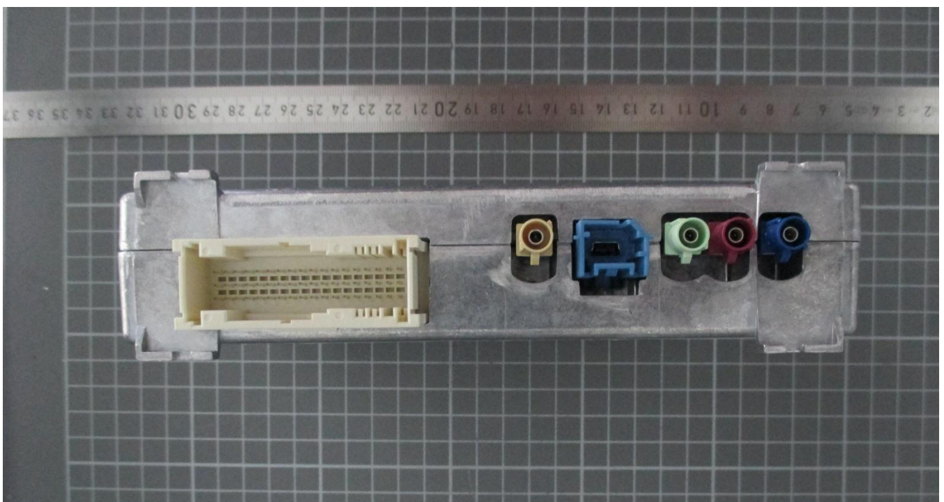
191350_10.JPG: Rear view with connectors
