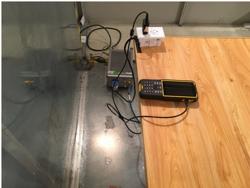
Line Conducted Side View
