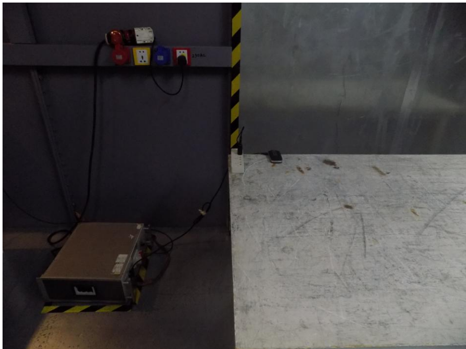
12.2.Photos of Conducted Emission test
