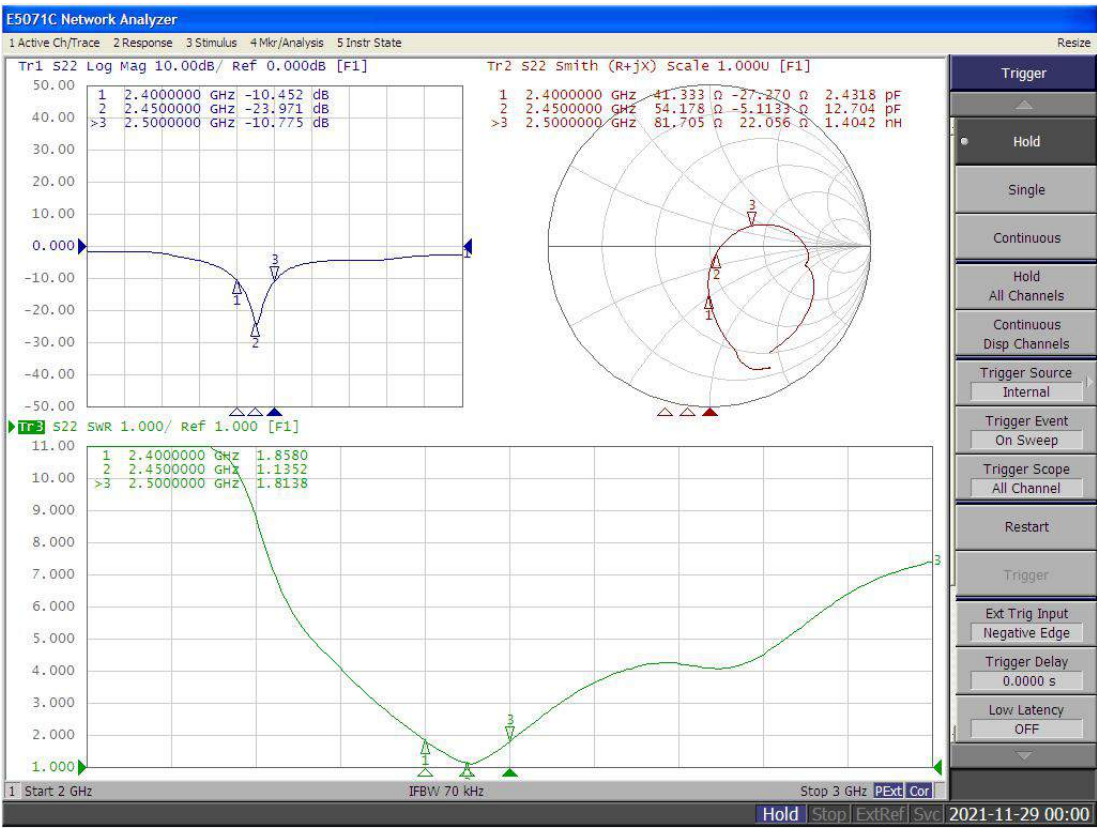
Figure 2 Antenna S parameters
