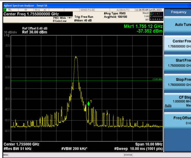
Band4-5MHz-QPSK-20375-1-5-High--37.35-PASS
