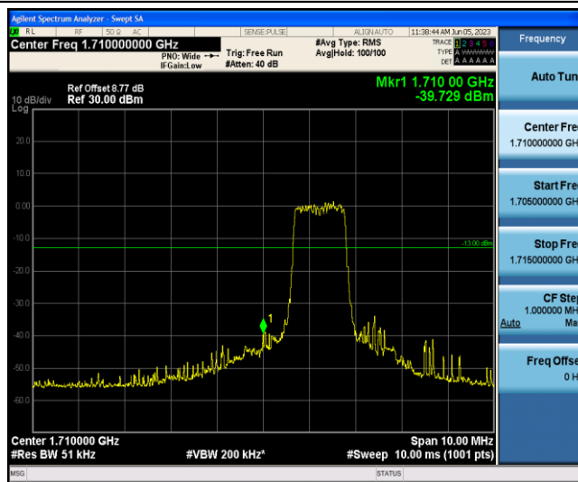
Band4-10MHz-QPSK-20000-6-0-Low--39.73-PASS
