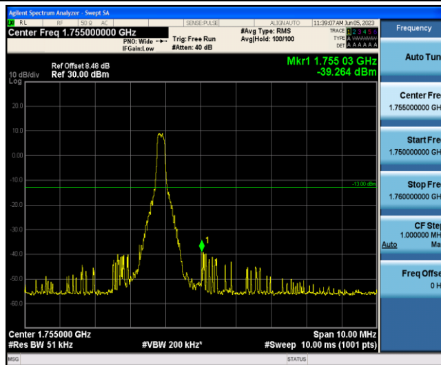
Band4-10MHz-QPSK-20350-1-5-High--39.26-PASS
