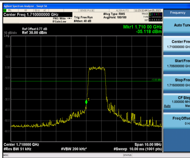
Band4-1.4MHz-QPSK-19957-6-0-Low--35.12-PASS
