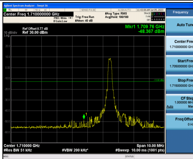
Band4-20MHz-16QAM-20050-1-0-Low--48.37-PASS
