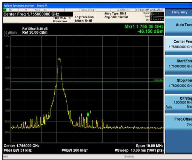
Band4-20MHz-16QAM-20300-1-5-High--46.15-PASS
