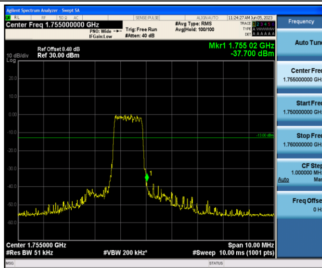
Band4-1.4MHz-16QAM-20393-6-0-High--37.70-PASS
