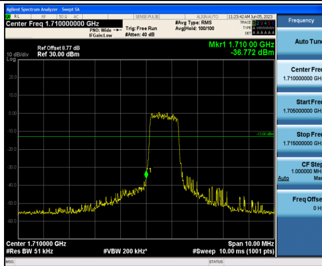
Band4-1.4MHz-16QAM-19957-6-0-Low--36.77-PASS
