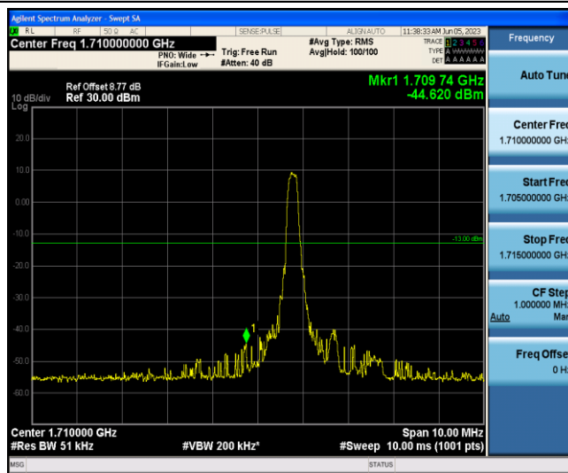
Band4-10MHz-16QAM-20000-1-0-Low--44.62-PASS
