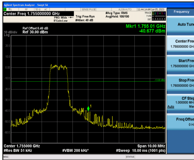
Band4-20MHz-16QAM-20300-6-0-High--40.68-PASS
