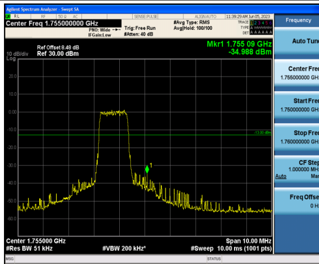
Band4-10MHz-QPSK-20350-6-0-High--34.99-PASS
