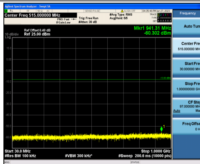
Band4-15MHz-16QAM-20175-1-0-Low-30-1000--60.3-PASS
