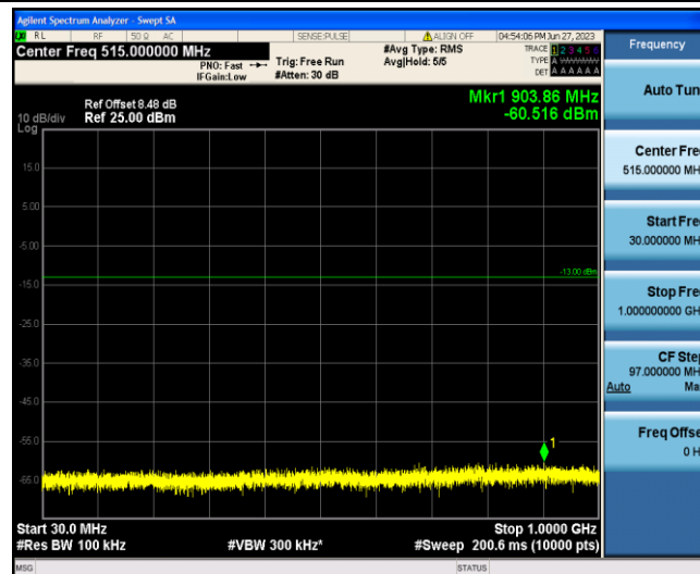
Band4-20MHz-QPSK-20175-1-0-Low-30-1000--60.52-PASS
