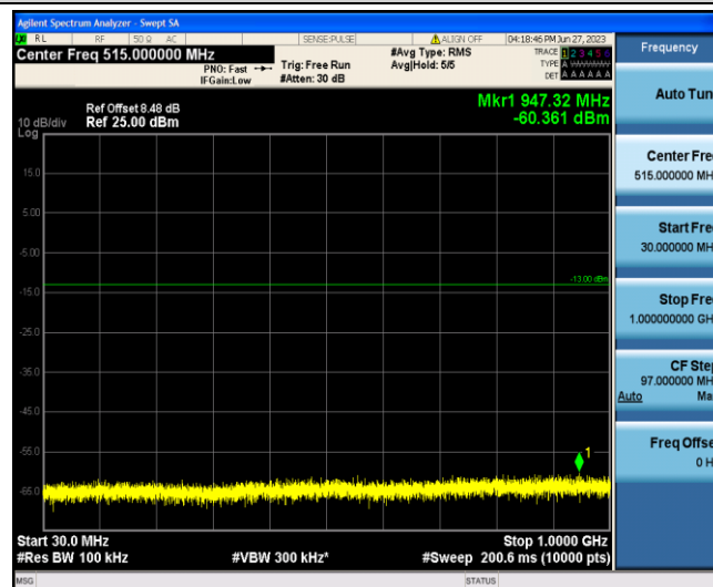
Band4-10MHz-QPSK-20175-1-0-Low-30-1000--60.36-PASS
