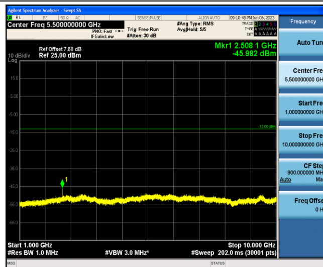
Band5-1.4MHz-QPSK-20525-1-0-Low-1000-10000--45.98-PASS
