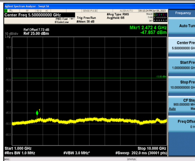
Band5-1.4MHz-16QAM-20407-1-0-Low-1000-10000--47.86-PASS
