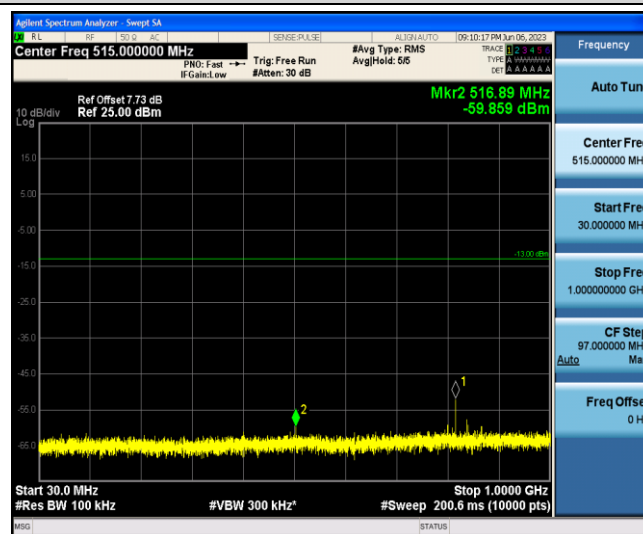
Band5-1.4MHz-16QAM-20407-1-0-Low-30-1000--59.86-PASS
