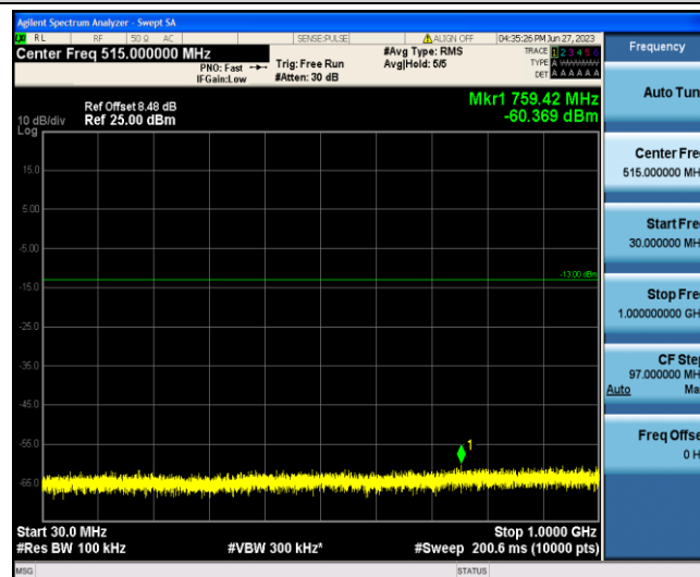
Band4-15MHz-QPSK-20175-1-0-Low-30-1000--60.37-PASS
