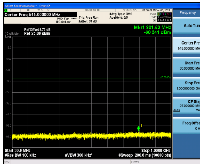
Band2-1.4MHz-16QAM-18607-1-0-Low-30-1000--60.34-PASS
