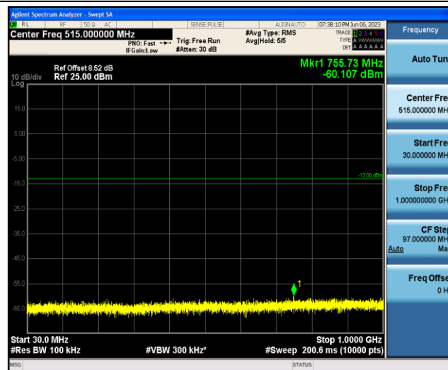
Band2-3MHz-QPSK-19185-1-0-Low-30-1000--60.11-PASS
