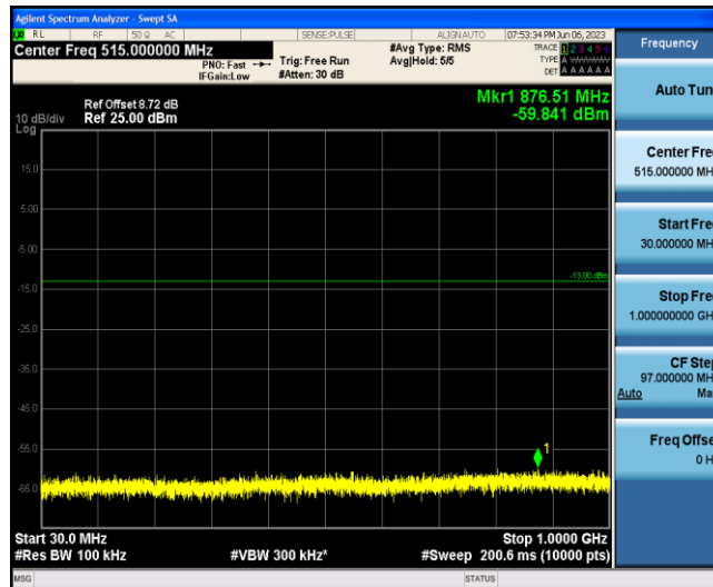
Band2-5MHz-QPSK-18625-1-0-Low-30-1000--59.84-PASS
