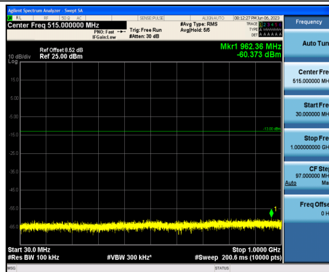
Band2-10MHz-QPSK-19150-1-0-Low-30-1000--60.37-PASS
