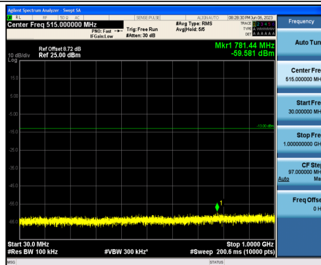
Band2-15MHz-QPSK-18900-1-0-Low-30-1000--59.58-PASS
