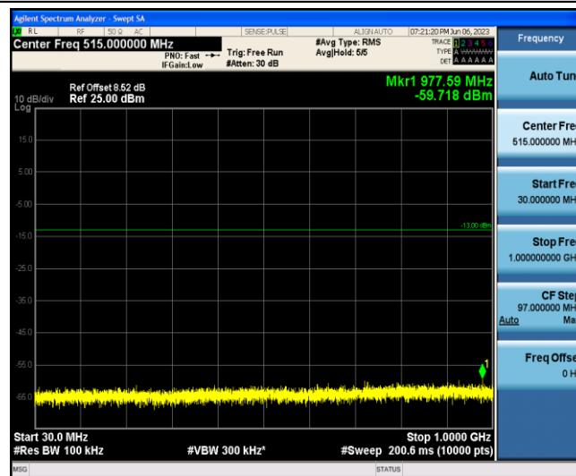
Band2-1.4MHz-QPSK-19193-1-0-Low-30-1000--59.72-PASS
