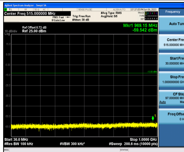
Band2-3MHz-16QAM-18615-1-0-Low-30-1000--59.54-PASS
