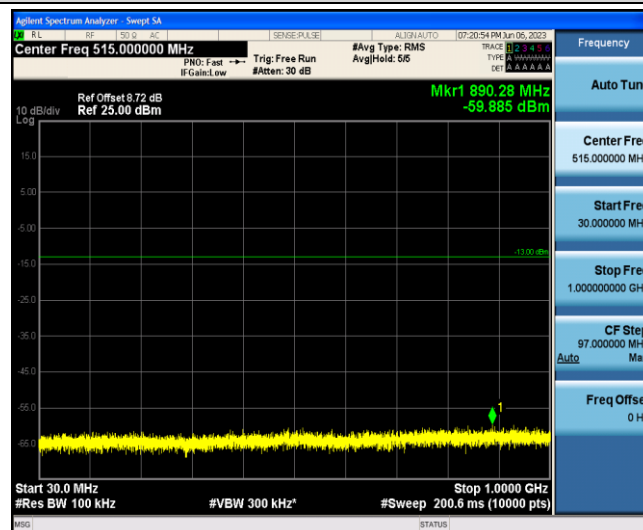
Band2-1.4MHz-16QAM-18900-1-0-Low-30-1000--59.89-PASS
