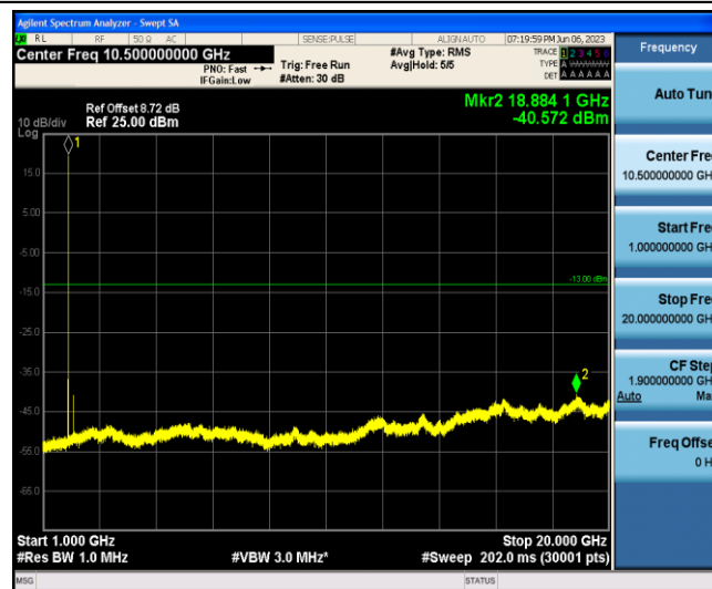
Band2-1.4MHz-QPSK-18607-1-0-Low-1000-20000--40.57-PASS
