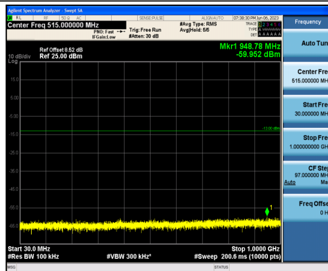
Band2-3MHz-16QAM-19185-1-0-Low-30-1000--59.95-PASS
