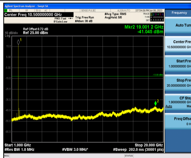
Band2-5MHz-16QAM-18625-1-0-Low-1000-20000--41.05-PASS
