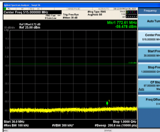
Band2-10MHz-16QAM-18900-1-0-Low-30-1000--59.48-PASS
