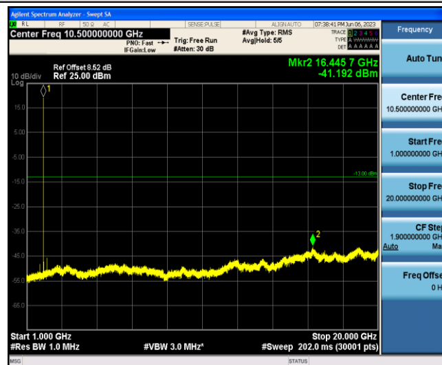
Band2-3MHz-16QAM-19185-1-0-Low-1000-20000--41.19-PASS
