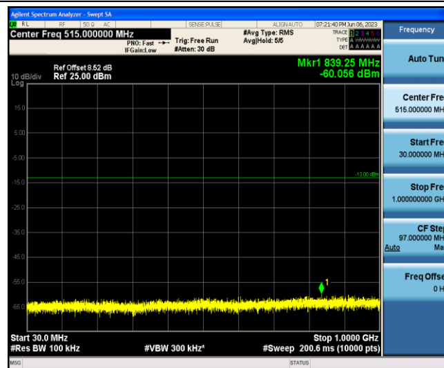
Band2-1.4MHz-16QAM-19193-1-0-Low-30-1000--60.06-PASS
