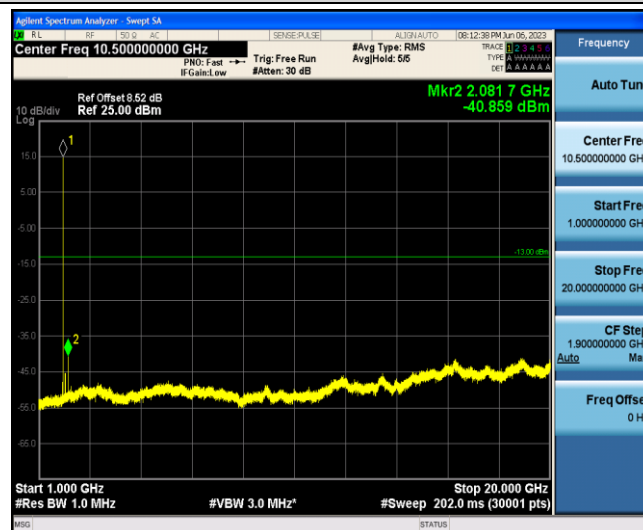
Band2-10MHz-QPSK-19150-1-0-Low-1000-20000--40.86-PASS
