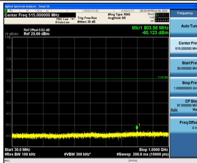
Band2-15MHz-QPSK-19125-1-0-Low-30-1000--60.12-PASS
