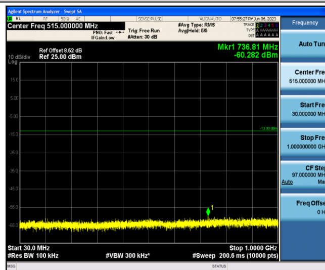
Band2-5MHz-16QAM-19175-1-0-Low-30-1000--60.28-PASS
