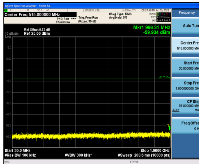
Band2-15MHz-QPSK-18675-1-0-Low-30-1000--59.93-PASS
