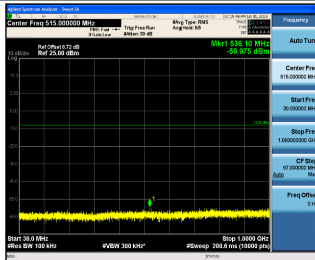
Band2-1.4MHz-QPSK-18607-1-0-Low-30-1000--59.98-PASS
