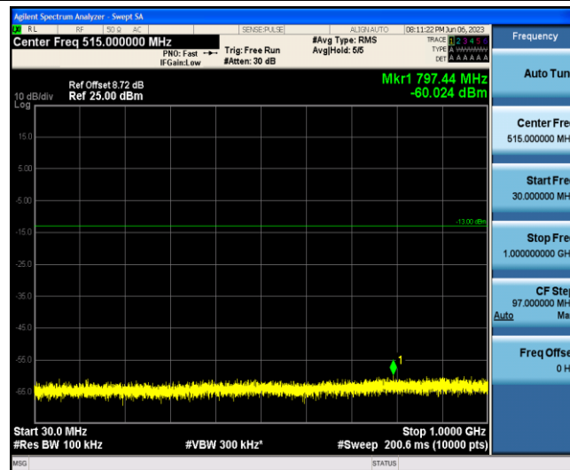
Band2-10MHz-16QAM-18650-1-0-Low-30-1000--60.02-PASS
