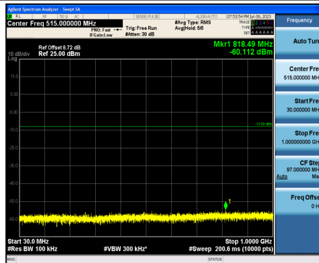
Band2-5MHz-16QAM-18625-1-0-Low-30-1000--60.11-PASS
