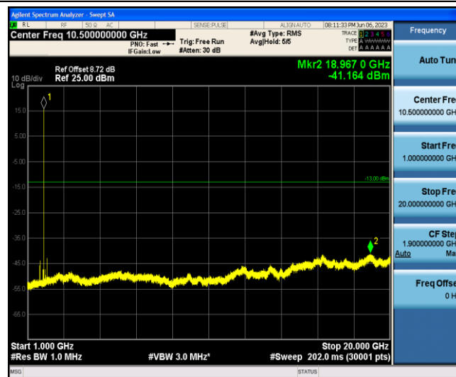
Band2-10MHz-16QAM-18650-1-0-Low-1000-20000--41.16-PASS
