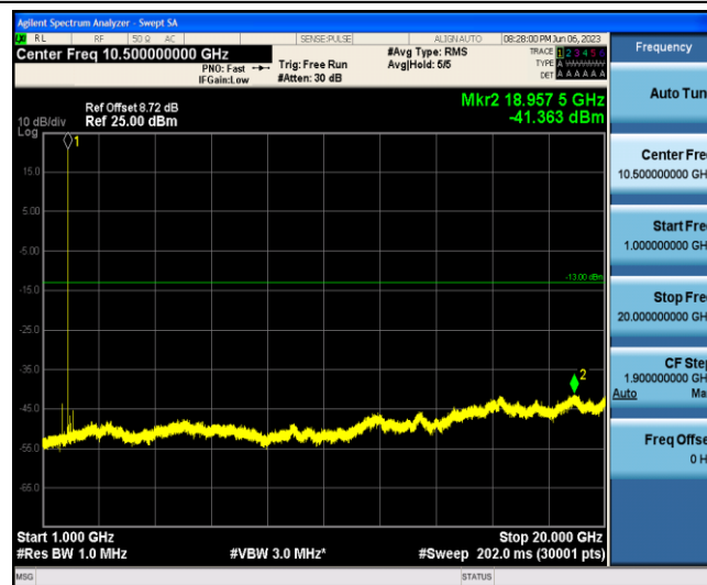
Band2-15MHz-QPSK-18675-1-0-Low-1000-20000--41.36-PASS
