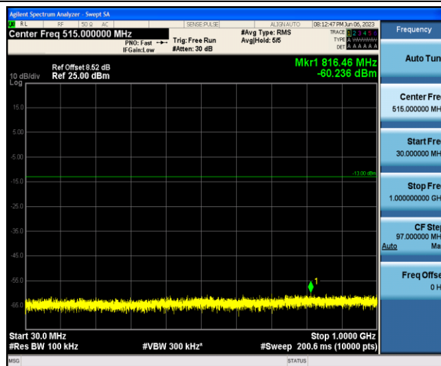
Band2-10MHz-16QAM-19150-1-0-Low-30-1000--60.24-PASS
