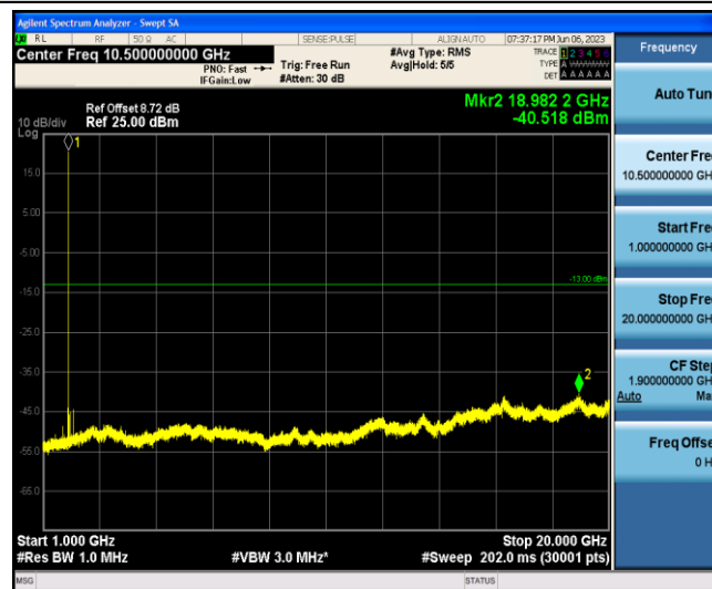
Band2-3MHz-16QAM-18615-1-0-Low-1000-20000--40.52-PASS
