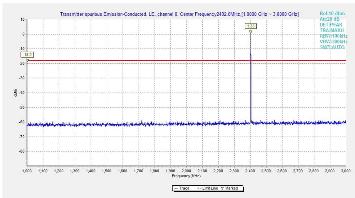
Fig.5. Transmitter Spurious Emission -Conducted: GFSK, 2402 MHz,1GHz - 3GHz
