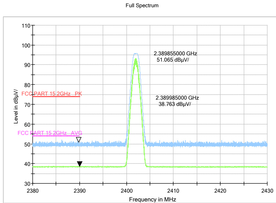
Fig.18. Transmitter Spurious Emission -Radiated (Power): BLE low channel
