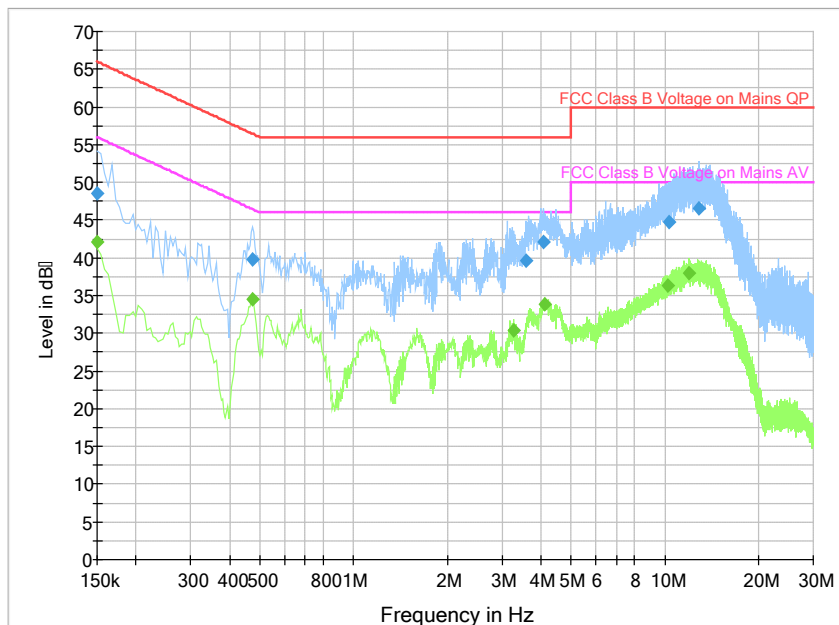
Fig.27. Conducted Emission from 150kHz to 30MHz
