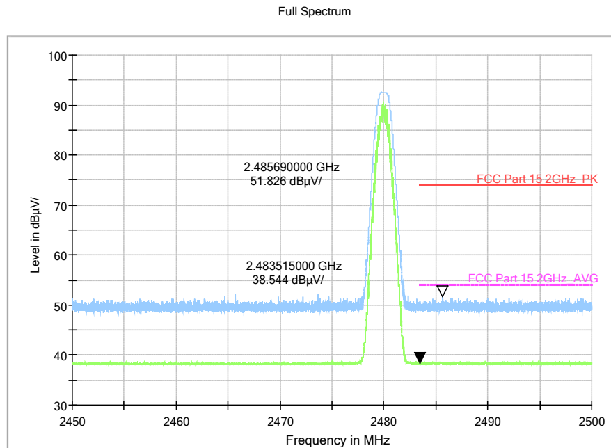
Fig.19. Transmitter Spurious Emission -Radiated (Power): BLE high channel
