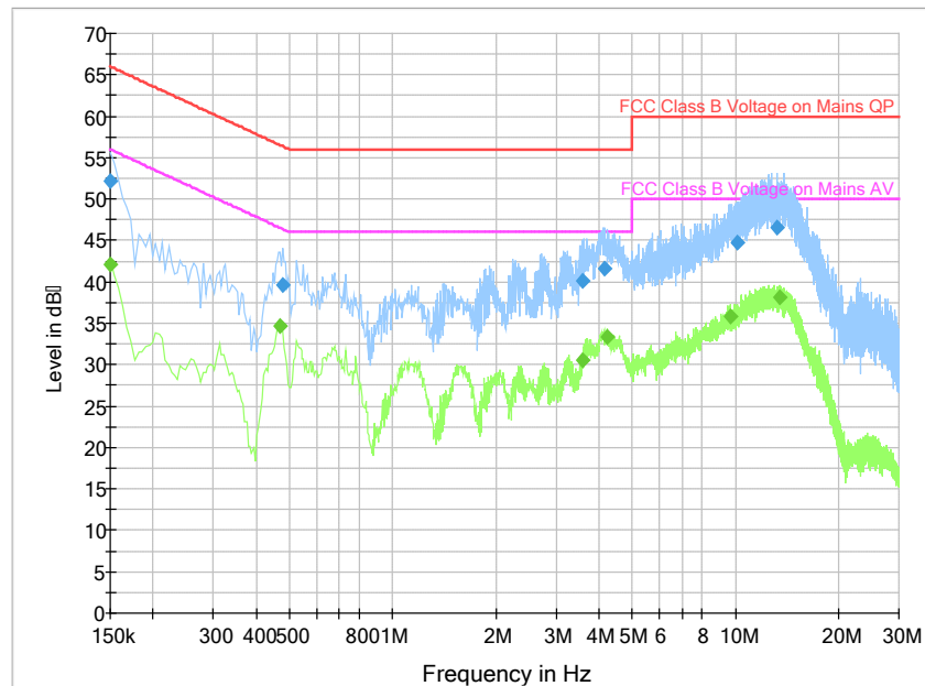
Fig.26. Conducted Emission from 150kHz to 30MHz
