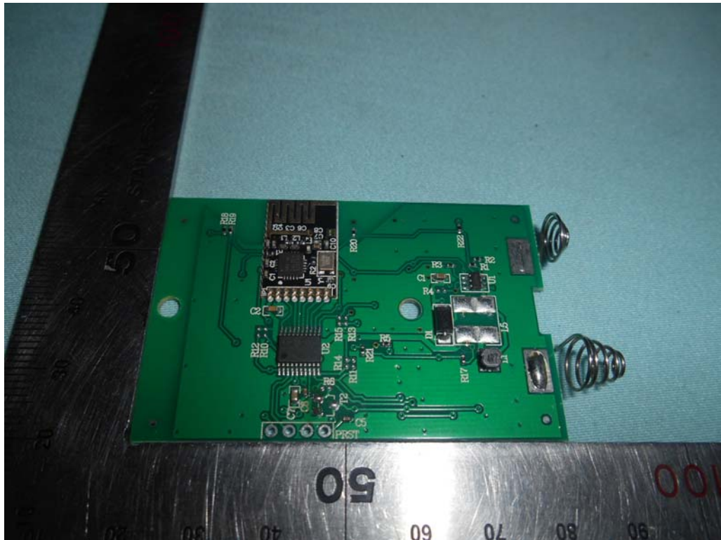
FIGURE 4 REMOTE CONTROL (M/N: WRC200T-01) KEYBOARD (FRONT VIEW)
