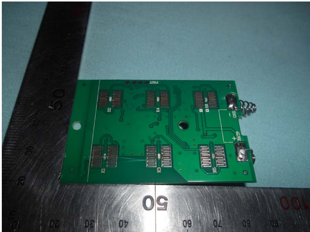
FIGURE 5 REMOTE CONTROL (M/N: WRC200T-01) KEYBOARD (BACK VIEW)
