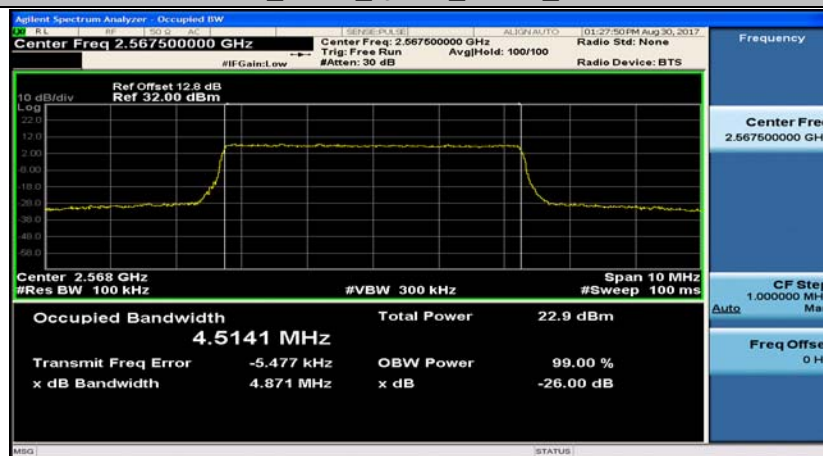
Band7_5MHz_16QAM_21425_25RB#0
