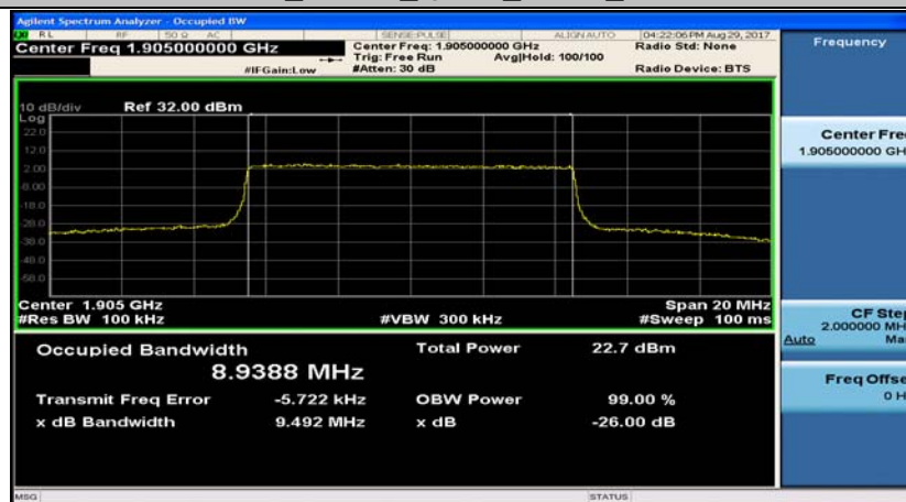
Band2_10MHz_16QAM_19150_50RB#0
