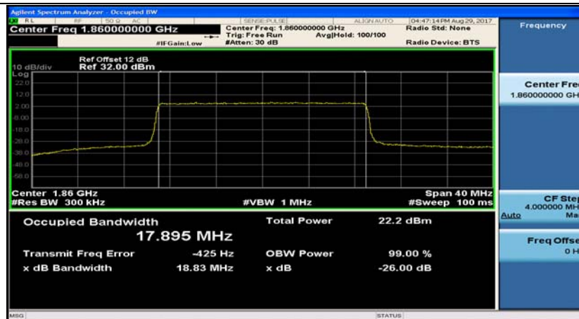
Band2_20MHz_16QAM_18700_100RB#0
