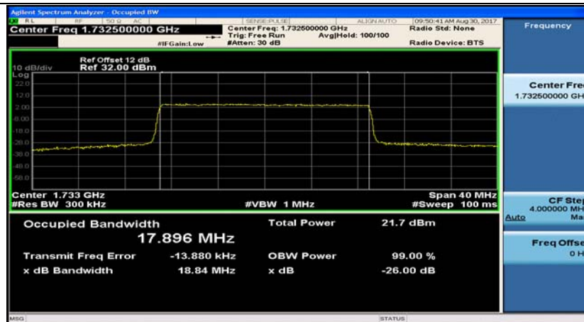
Band4_20MHz_QPSK_20300_100RB#0
