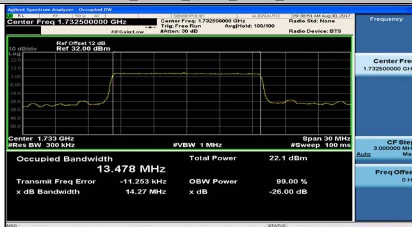
Band4_15MHz_16QAM_20175_75RB#0
