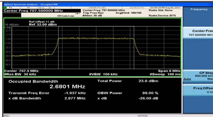
Band12_3MHz_QPSK_23165_15RB#0
