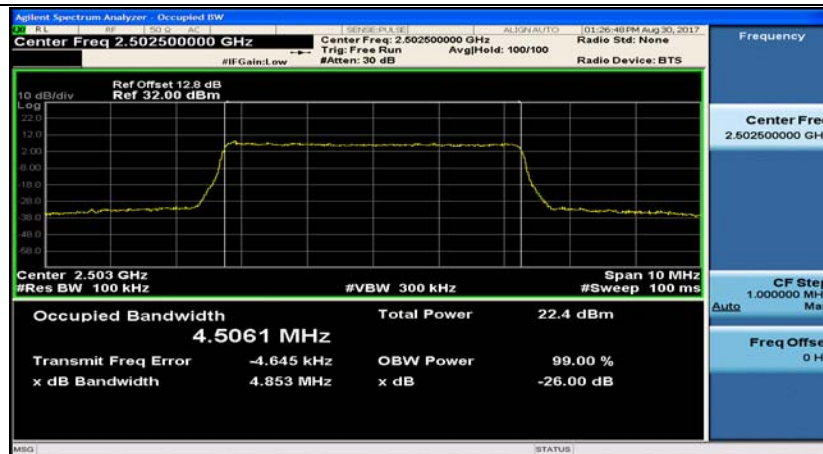
Band7_5MHz_16QAM_20775_25RB#0
