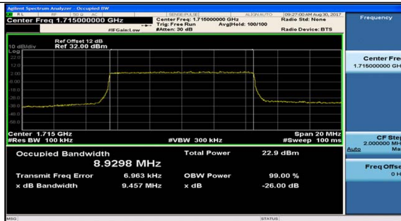
Band4_10MHz_16QAM_20000_50RB#0
