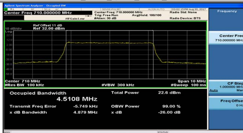
Band17_5MHz_16QAM_23790_25RB#0
