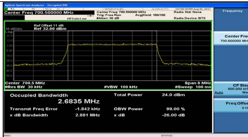
Band12_3MHz_16QAM_23025_15RB#0
