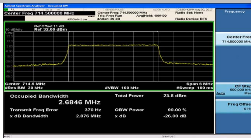
Band12_3MHz_16QAM_23165_15RB#0
