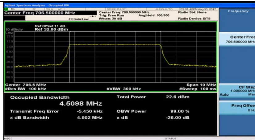
Band17_5MHz_16QAM_23755_25RB#0
