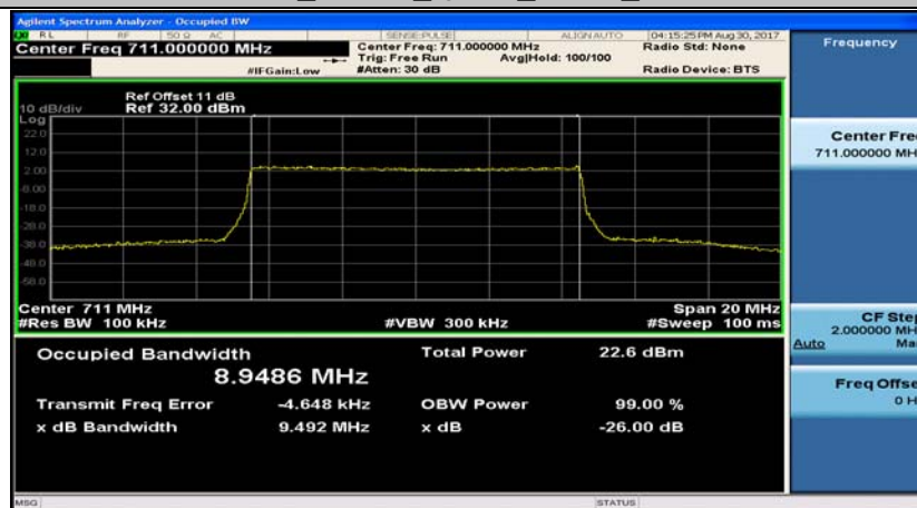
Band12_10MHz_16QAM_23130_50RB#0
