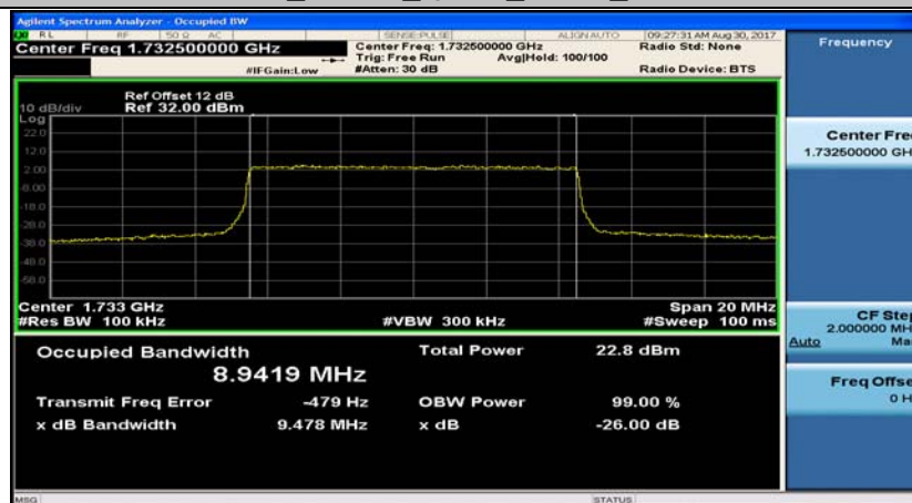
Band4_10MHz_16QAM_20175_50RB#0
