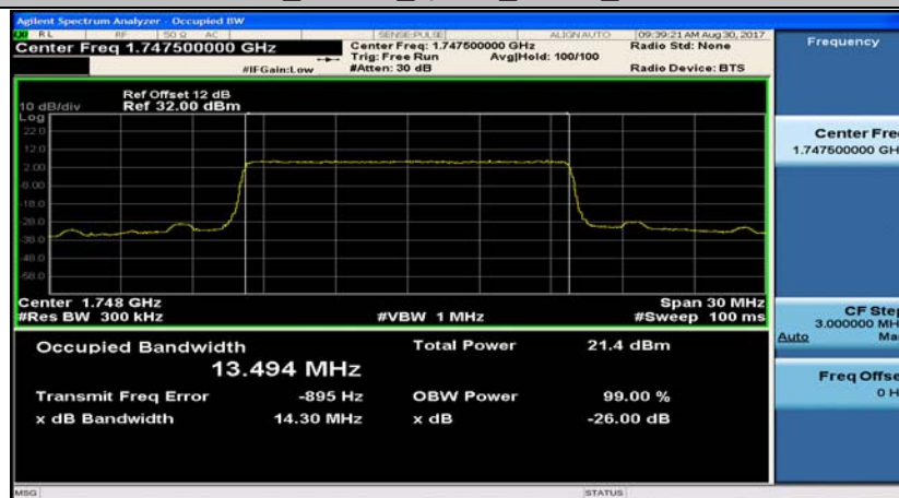
Band4_15MHz_16QAM_20325_75RB#0
