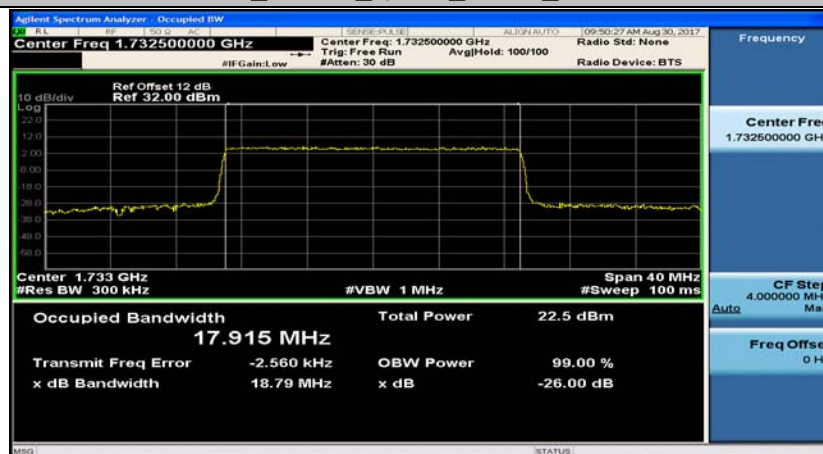
Band4_20MHz_16QAM_20175_100RB#0
