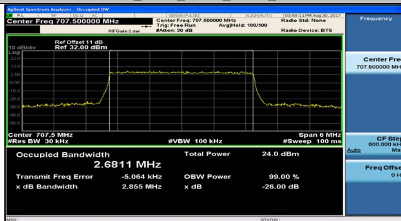
Band12_3MHz_16QAM_23095_15RB#0
