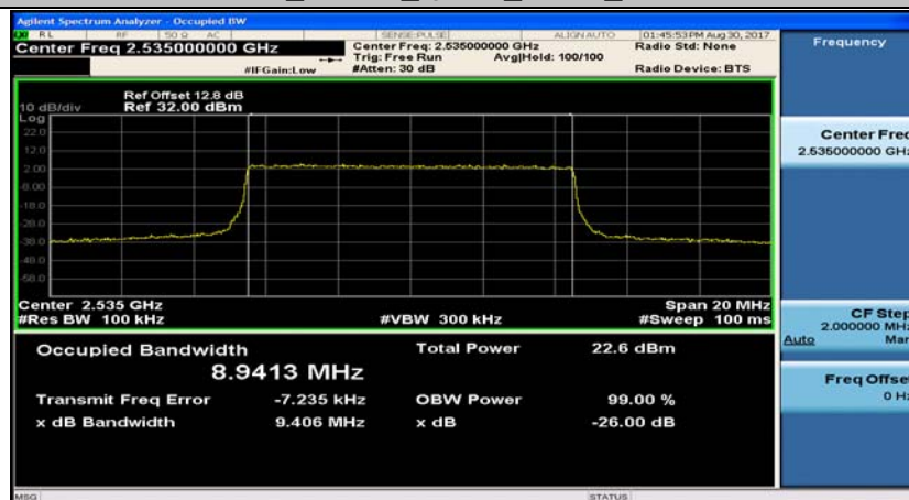
Band7_10MHz_16QAM_21100_50RB#0
