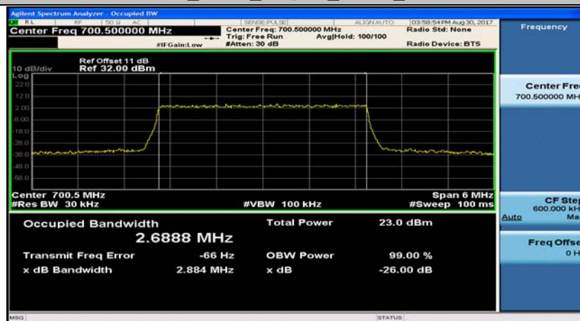
Band12_3MHz_QPSK_23095_15RB#0
