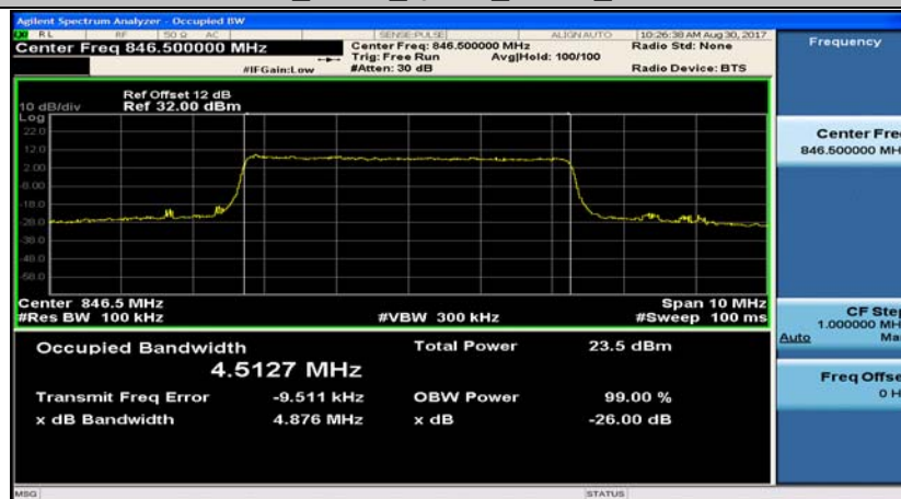
Band5_5MHz_16QAM_20625_25RB#0
