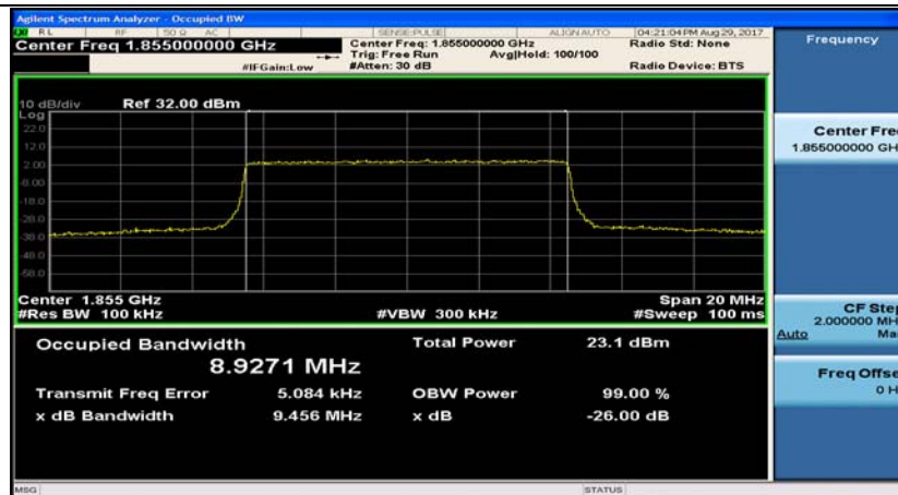
Band2_10MHz_16QAM_18650_50RB#0
