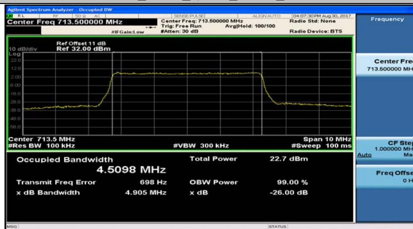
Band12_5MHz_16QAM_23155_25RB#0
