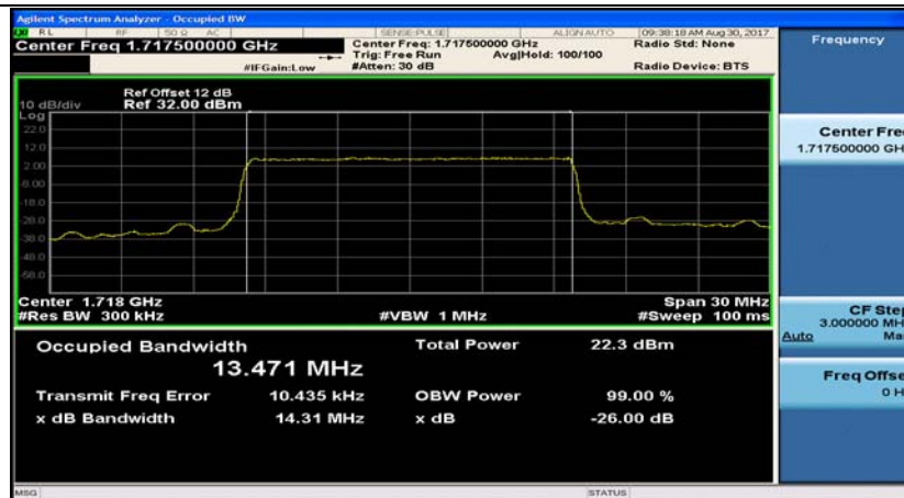
Band4_15MHz_16QAM_20025_75RB#0
