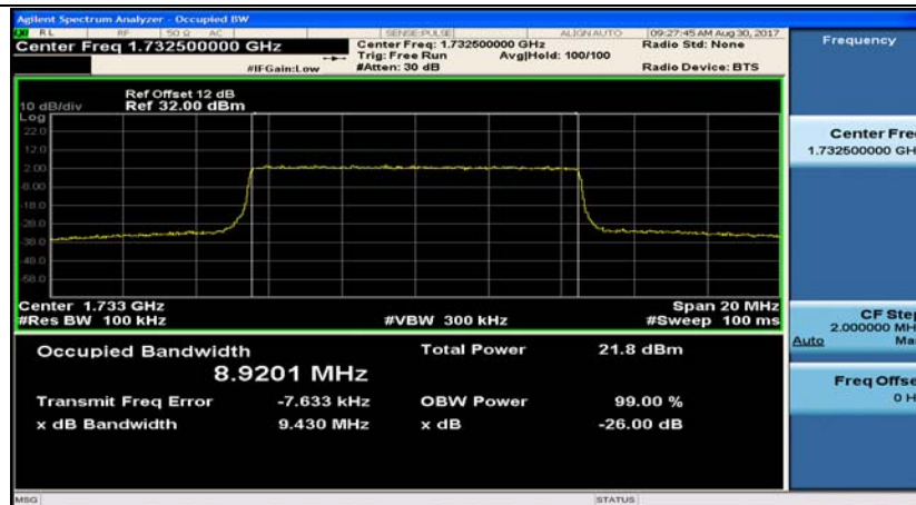
Band4_10MHz_QPSK_20350_50RB#0
