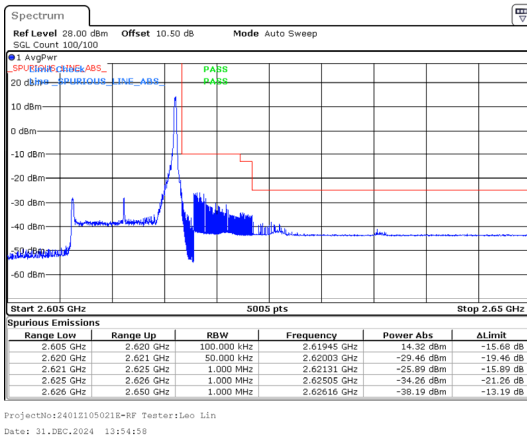
Band 38 10MHz/2615.0/High QPSK 1@49
