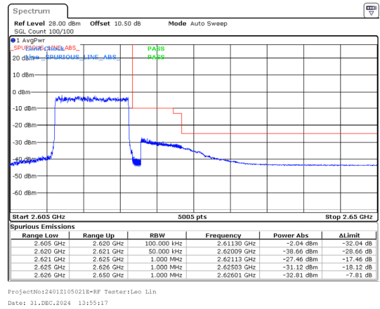
Band 38 10MHz/2615.0/High QPSK 50@0
