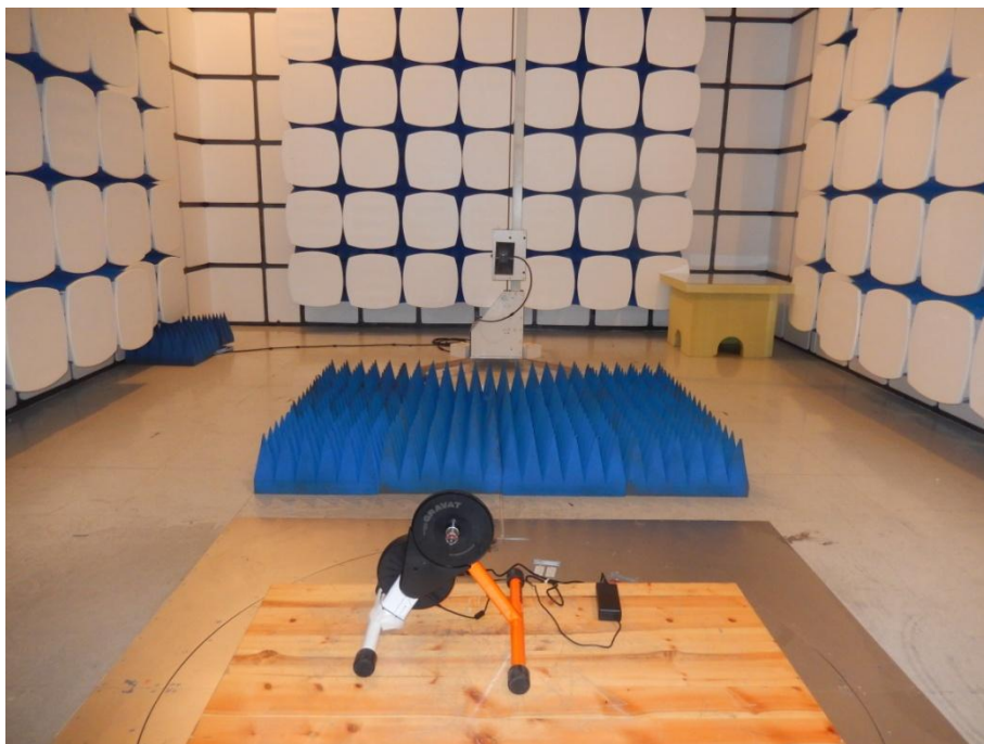
FCC radiation H
