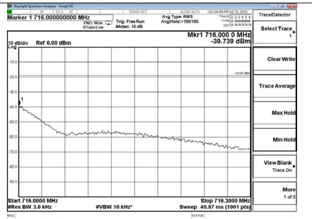
Lower 700MHz band GSM UL Right Side 10dB Above AGC
