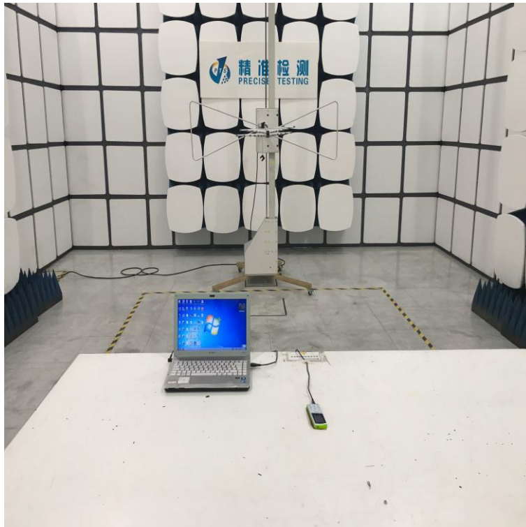
FCC RADIATED EMISSION TEST SETUP
