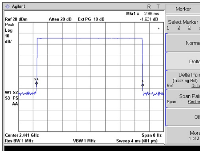
DH5/2-DH5/3-DH5
