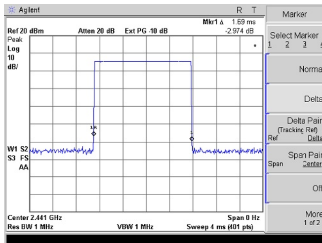
DH3/2-DH3/3-DH3
