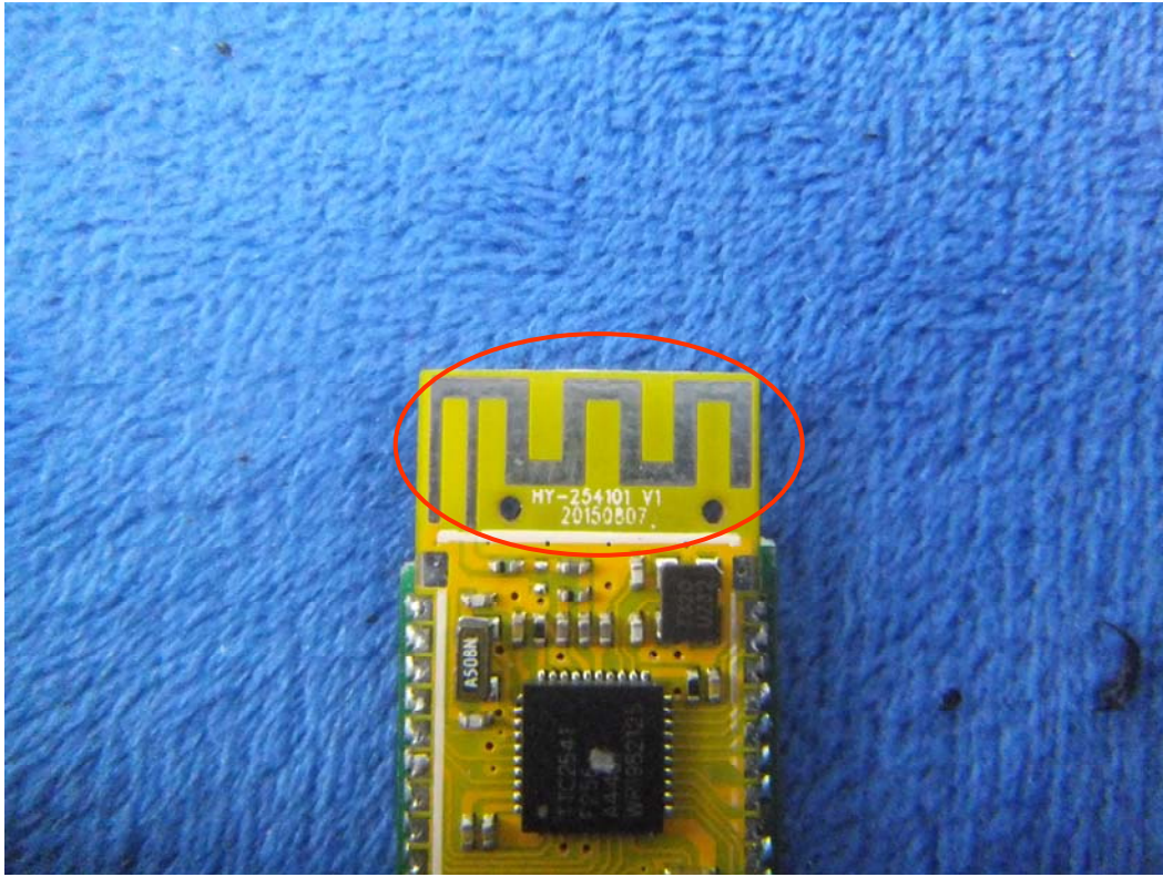
Antenna View
