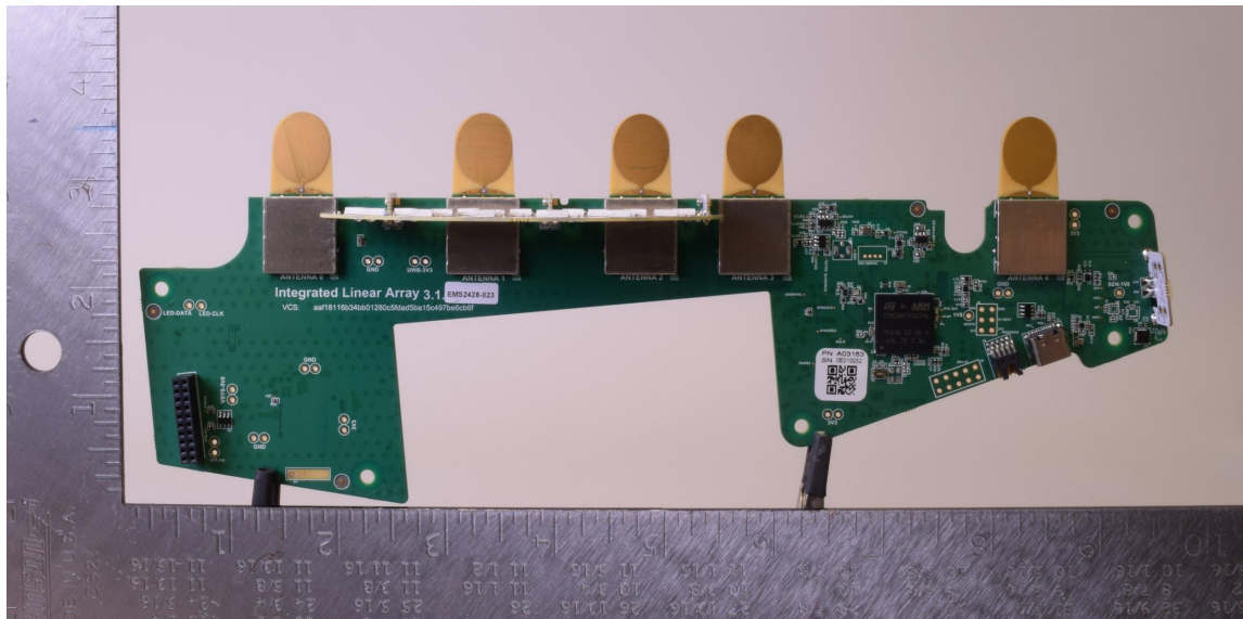
Figure 2: LP203 showing antenna
