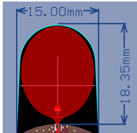
Figure 1: Individual Antenna Dimensions
