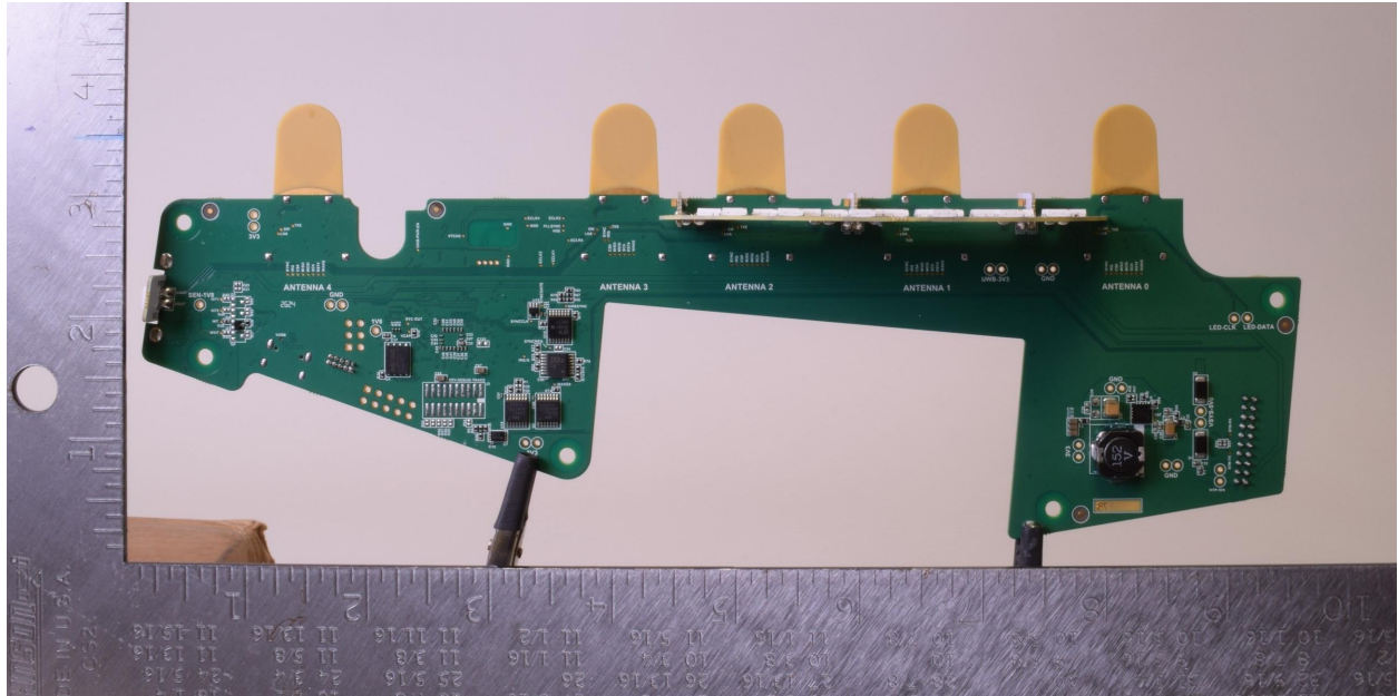
LP203: Back
