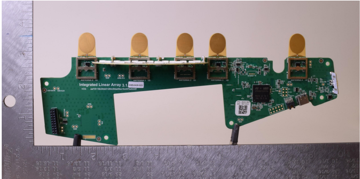
LP203: Front without Shields
