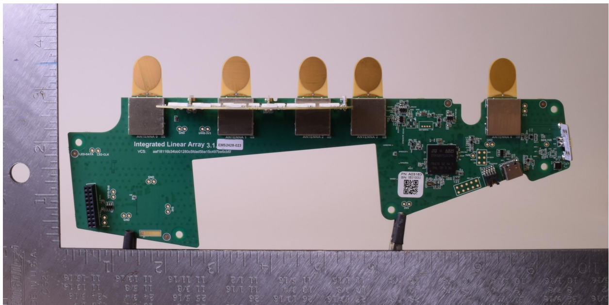
LP203: Front
