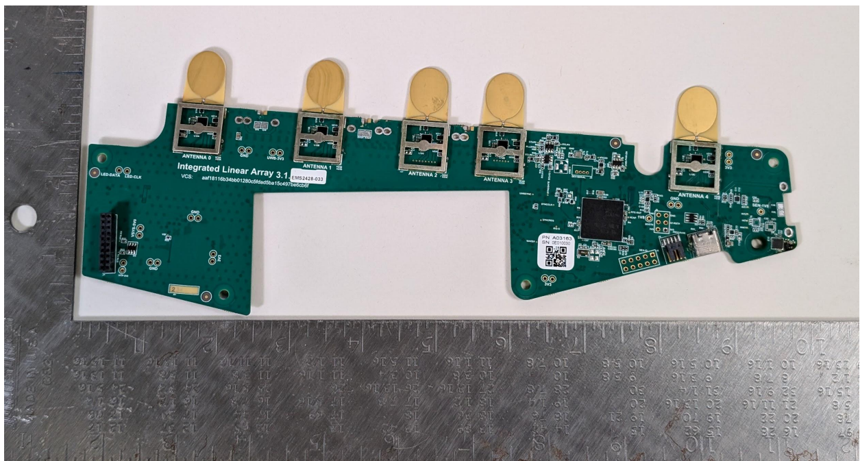
LP203: Front without Shields and LED boards*
