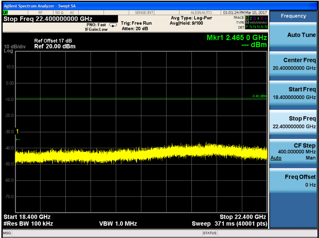
Figure 16: Spurious Emissions BT Mode
