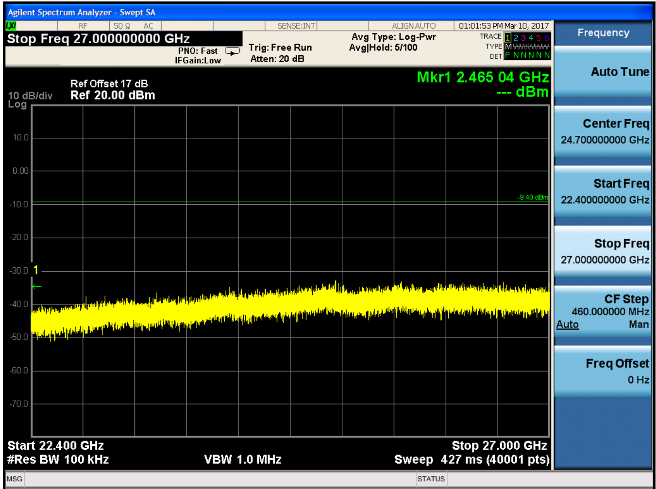
Figure 17: Spurious Emissions BT Mode `
