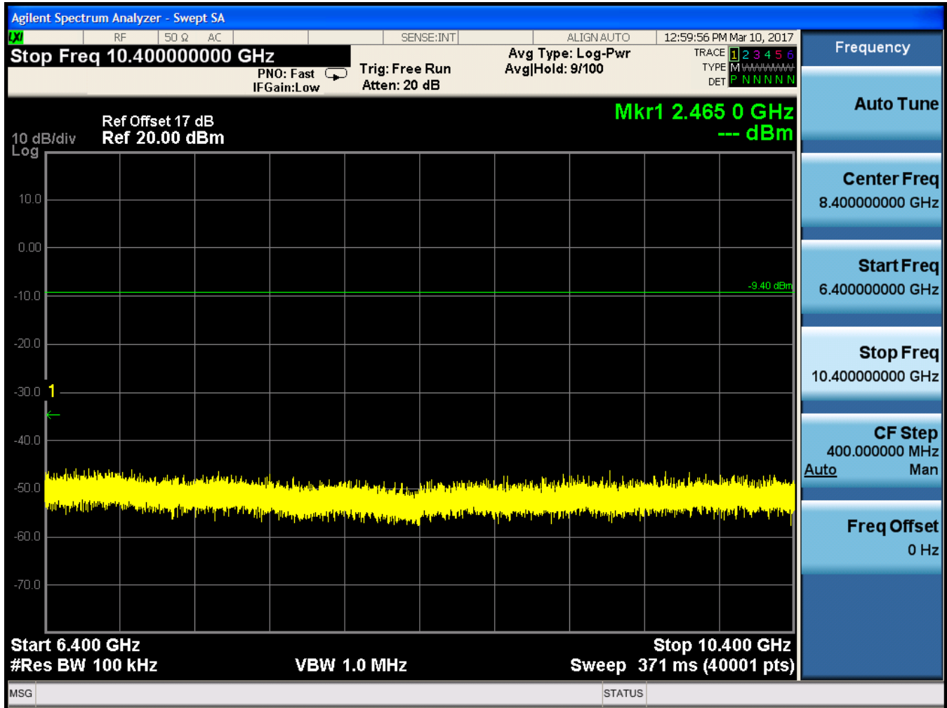
Figure 13: Spurious Emissions BT Mode
