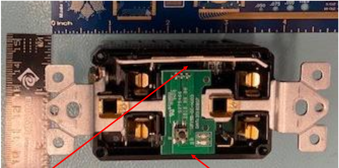
Wire antenna
