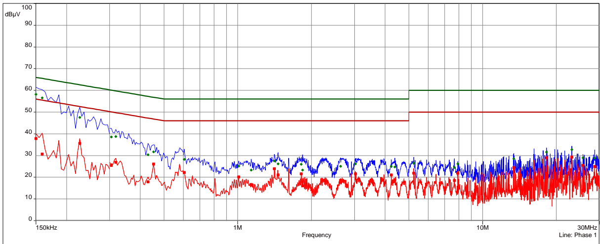
CISPR 22/CISPR22B
