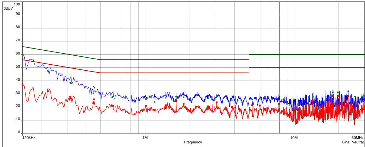
CISPR 22/CISPR22B
