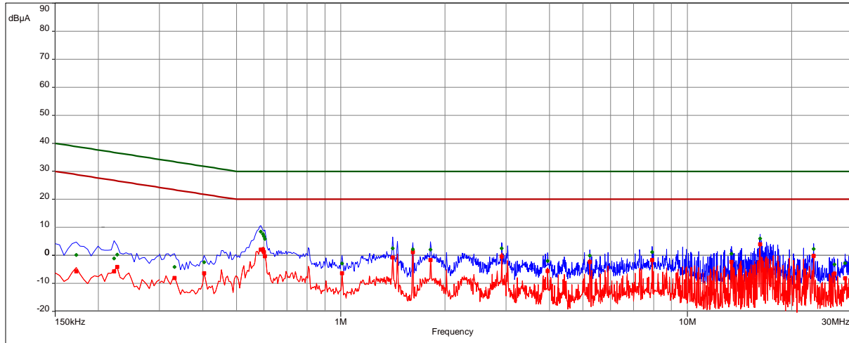
CISPR 22/CISPR 22B
