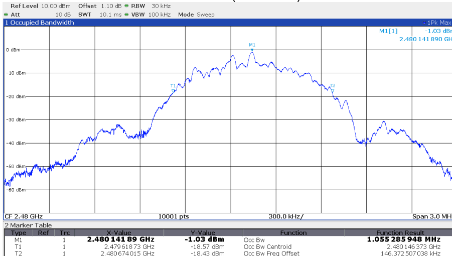
Channel 39 (2480 MHz)
