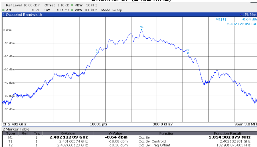
Channel 37 (2402 MHz)
