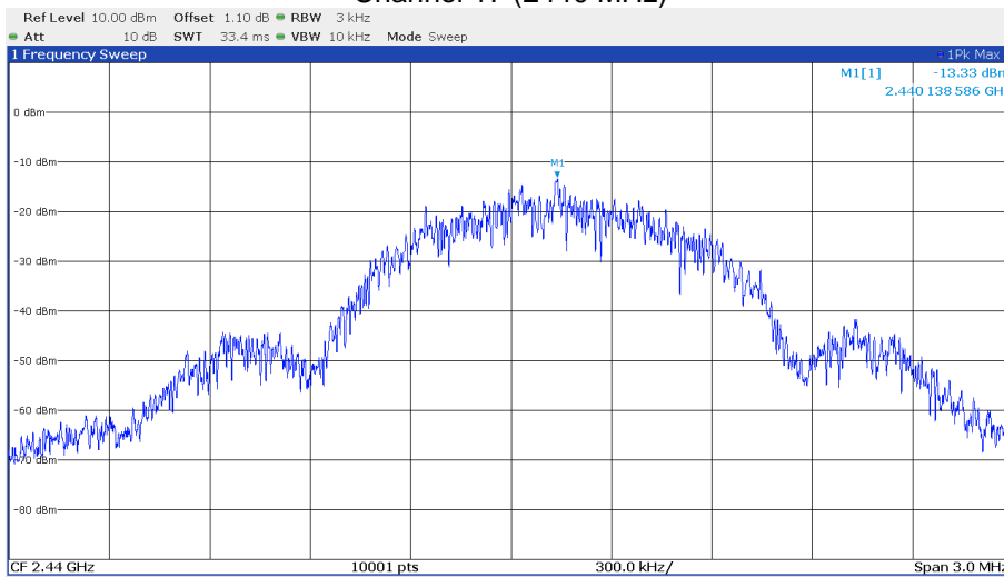
Channel 17 (2440 MHz)
