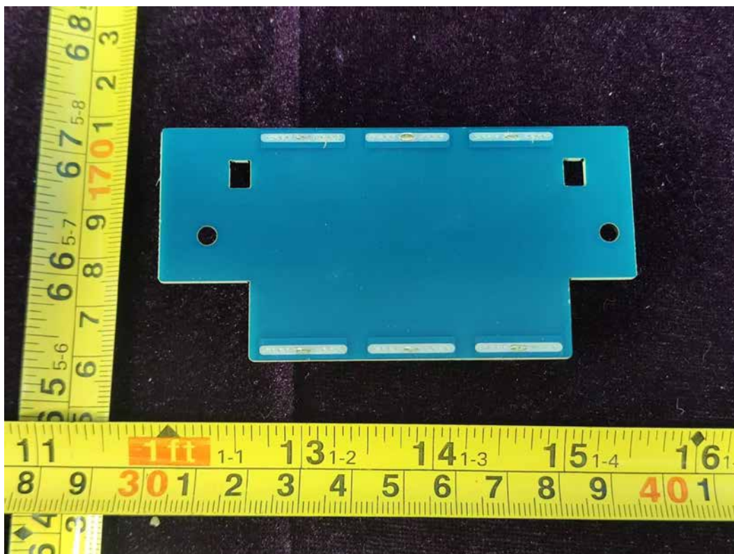
FIGURE 45 SWI331 WIRELESS (M/N: SWI331 WIRELESS-020) BOARD1-1
