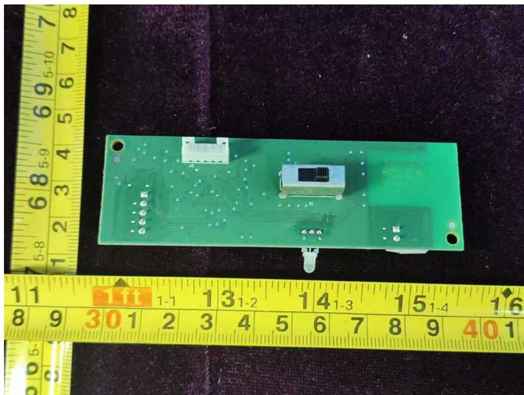
FIGURE 15 SWI331 WIRELESS (M/N: SWI331 WIRELESS-002) BOARD2-3
