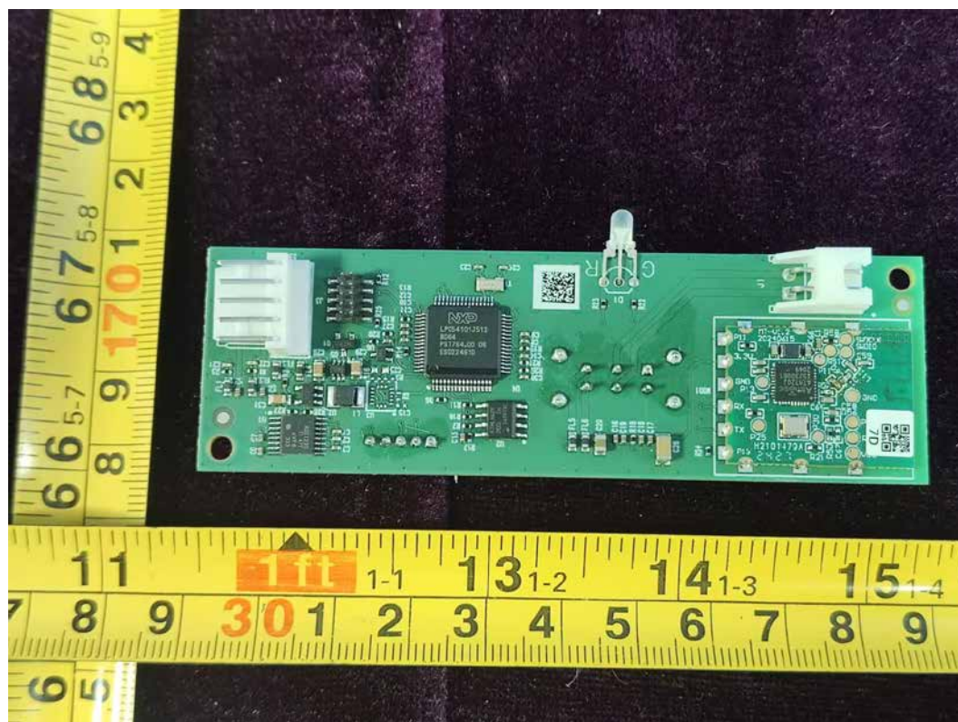
FIGURE 30 SWI331 WIRELESS (M/N: SWI331 WIRELESS-008) BOARD2-1
