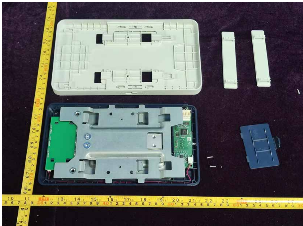
FIGURE 26 SWI331 WIRELESS (M/N: SWI331 WIRELESS-008) COVER REMOVE-2
