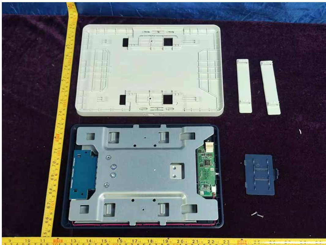
FIGURE 43 SWI331 WIRELESS (M/N: SWI331 WIRELESS-020) COVER REMOVE-2
