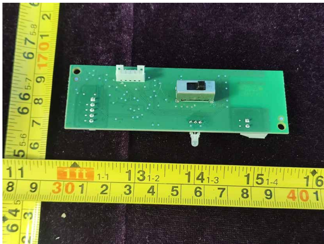
FIGURE 49 SWI331 WIRELESS (M/N: SWI331 WIRELESS-020) BOARD2-3
