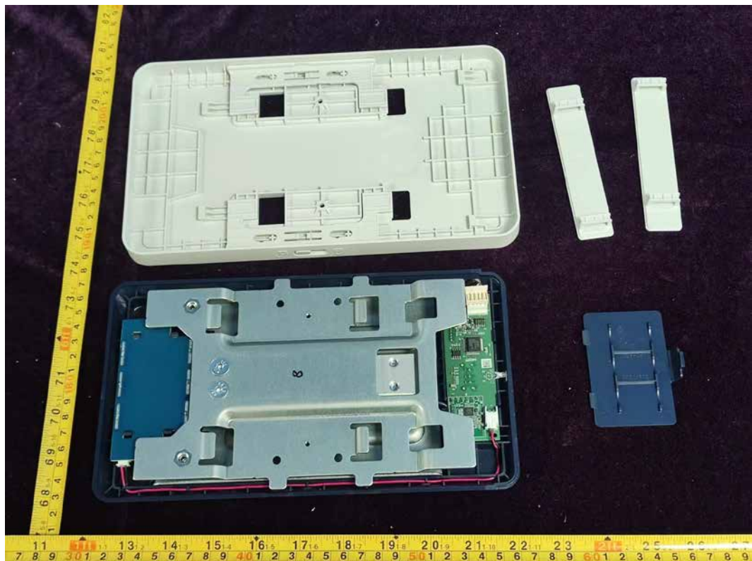
FIGURE 9 SWI331 WIRELESS (M/N: SWI331 WIRELESS-002) COVER REMOVE-2
