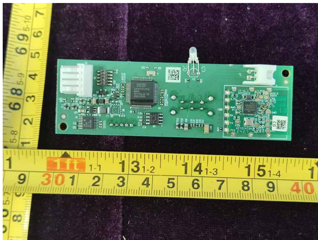
FIGURE 13 SWI331 WIRELESS (M/N: SWI331 WIRELESS-002) BOARD2-1
