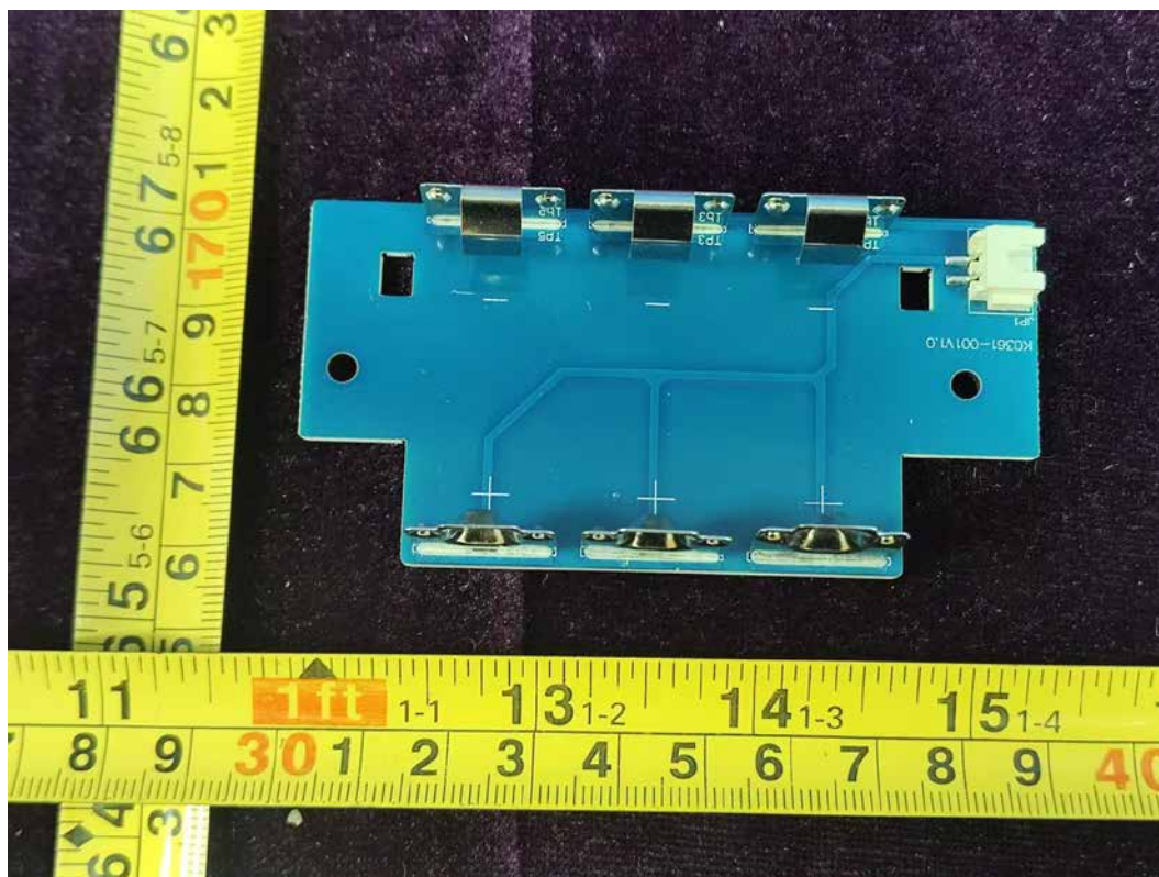
FIGURE 47 SWI331 WIRELESS (M/N: SWI331 WIRELESS-020) BOARD2-1
