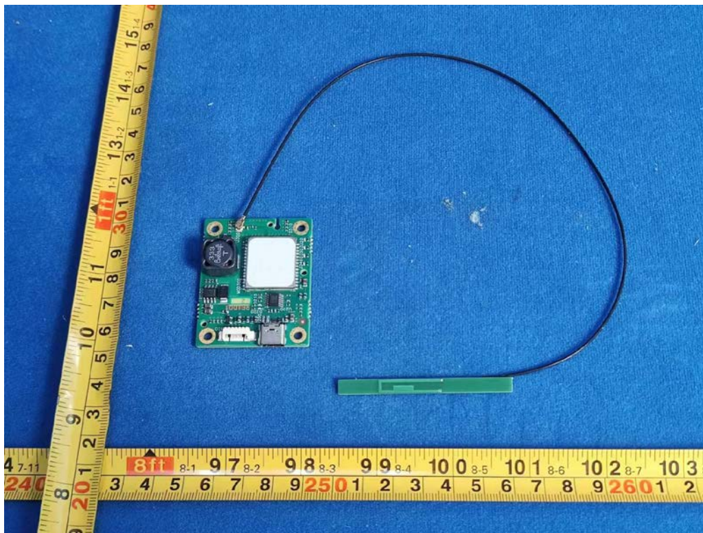
FIGURE 2 RF MODULE (MT-UHF-RFID01) BACK APPEARANCE (SHIPPED WITH ANT1)
