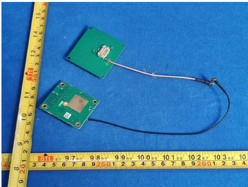
FIGURE 4 RF MODULE (MT-UHF-RFID01) BACK APPEARANCE (SHIPPED WITH ANT2)
