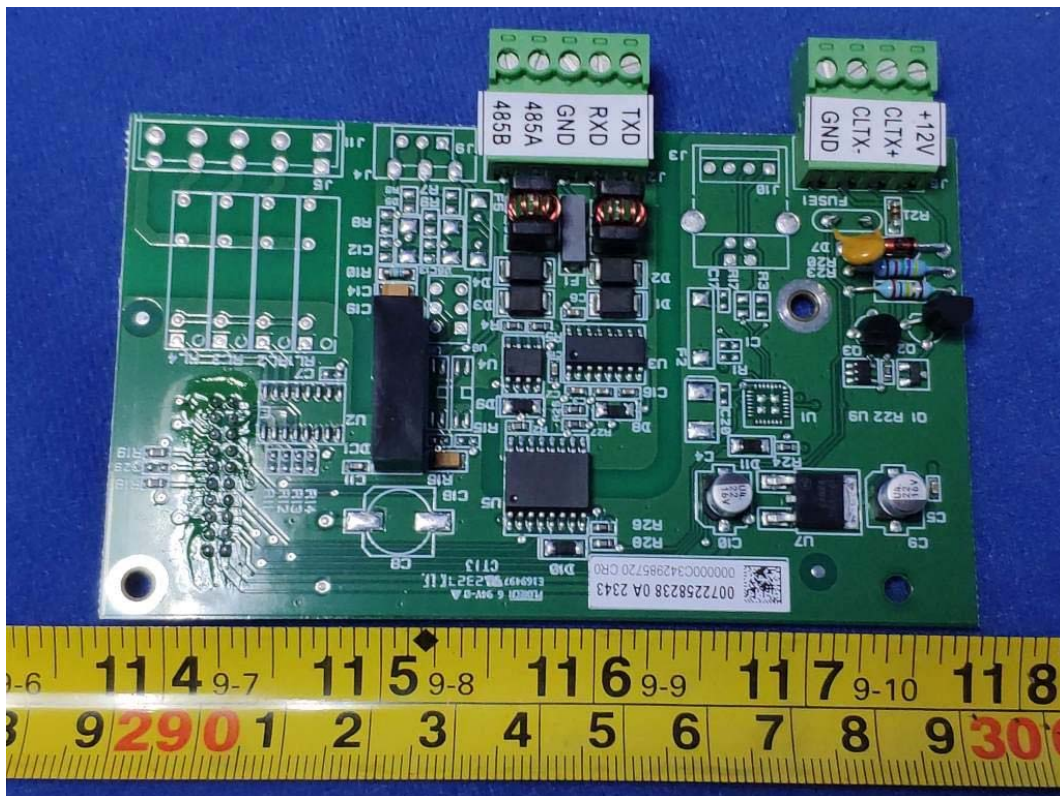
FIGURE 14 IND246 (IND246) CONTROL BOARD FRONT
