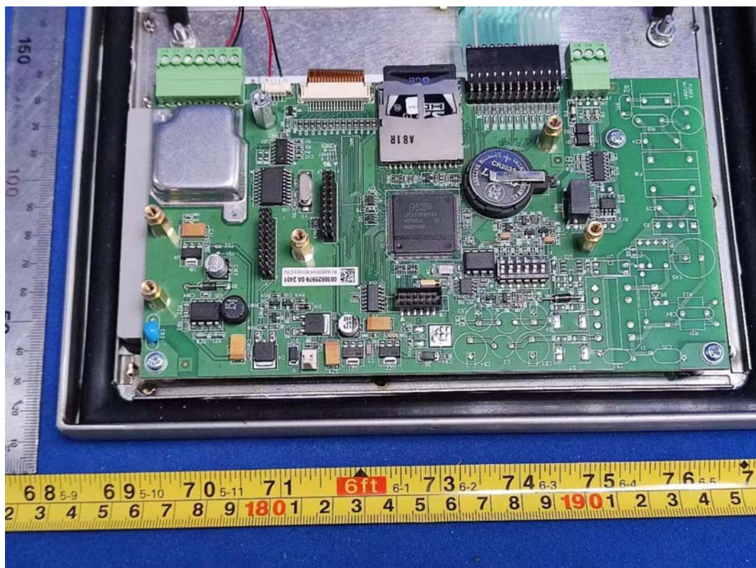
FIGURE 16 IND246 (IND246) POWER BOARD
