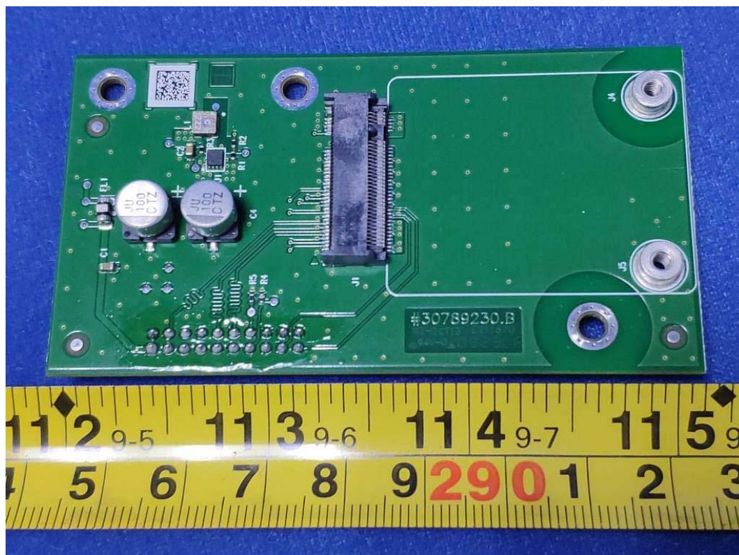
FIGURE 12 IND246 (IND246) SWITCH BOARD FRONT
