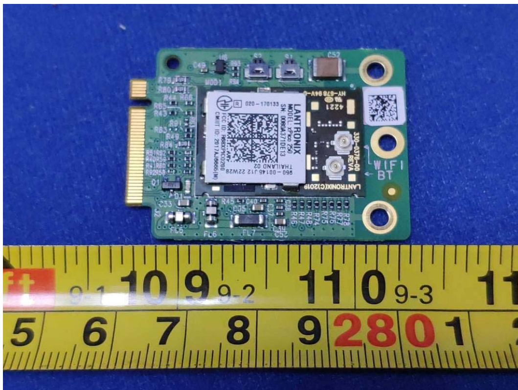
FIGURE 8 IND246 (IND246) RF BOARD FRONT
