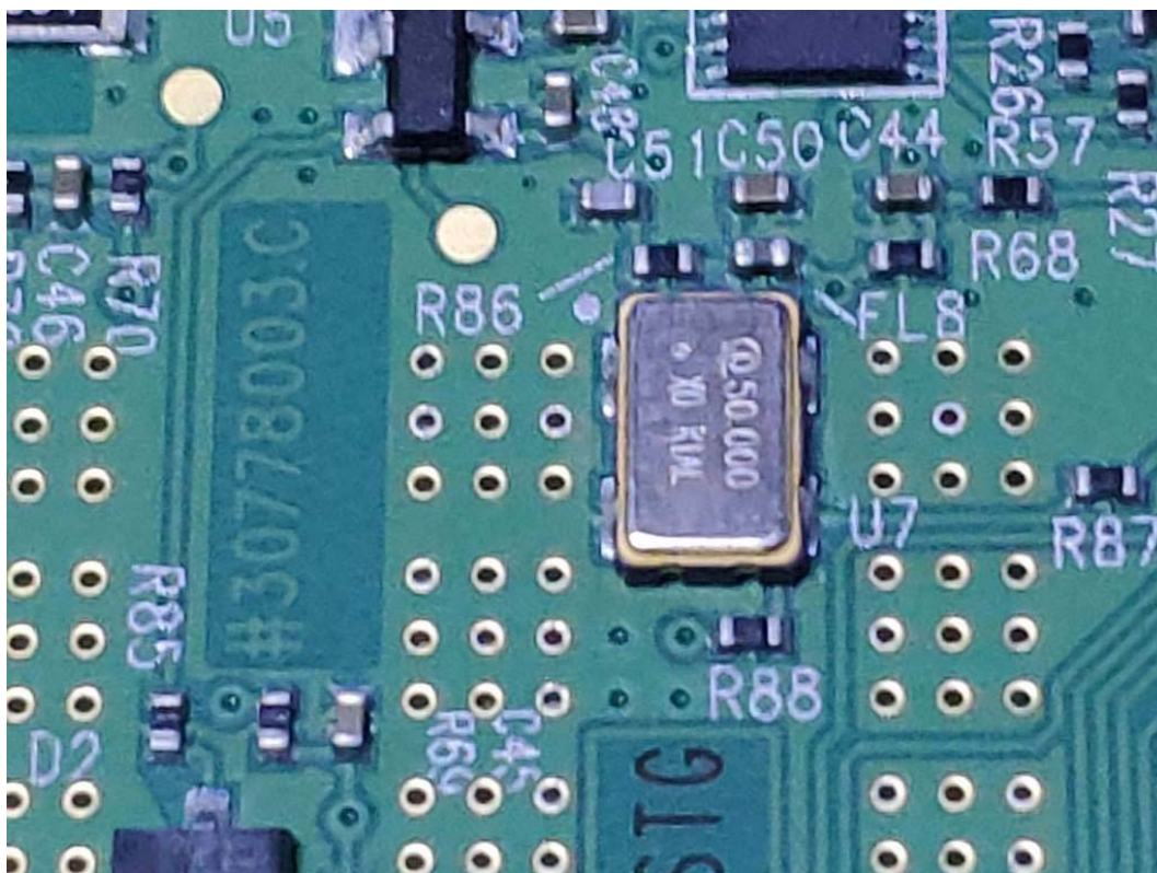
FIGURE 10 IND246 (IND246) CHIP & CRYSTAL ON RF BOARD
