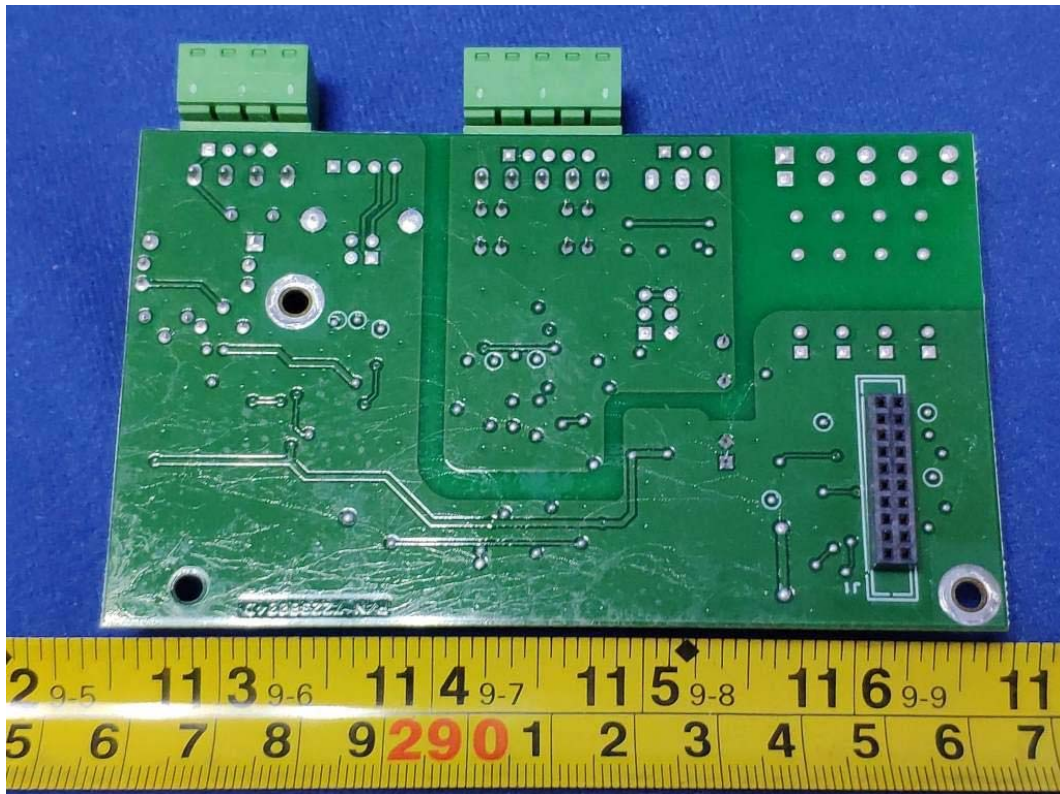
FIGURE 15 IND246 (IND246) CONTROL BOARD BACK
