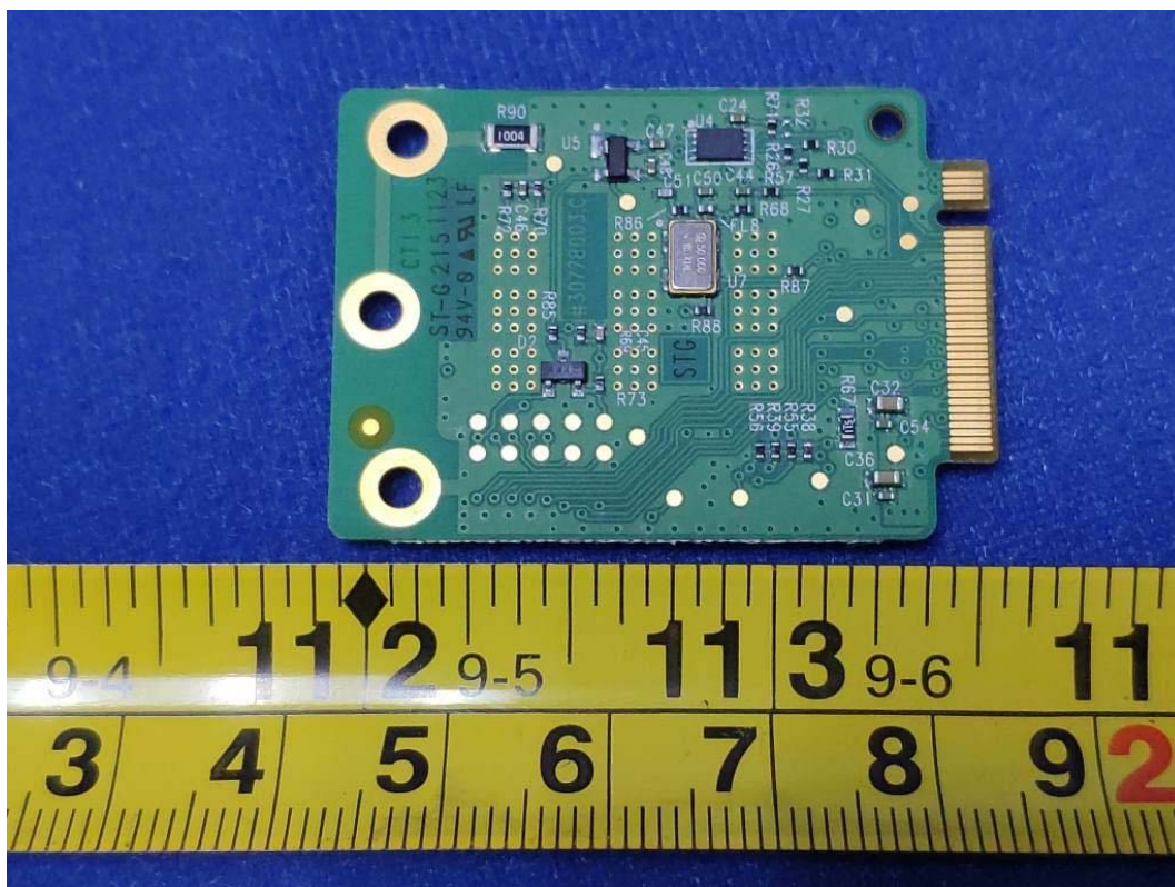
FIGURE 9 IND246 (IND246) RF BOARD BACK
