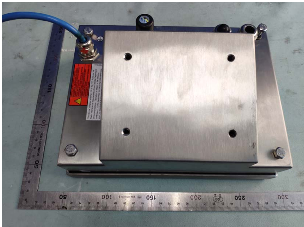
FIGURE 6 WEIGHING TERMINAL (M/N: IND256x) GENERAL APPEARANCE (BOTTOM VIEW)
