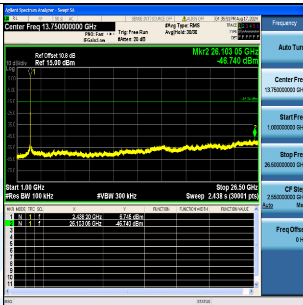
11G-Ant2-2437-1000~26500-PASS
