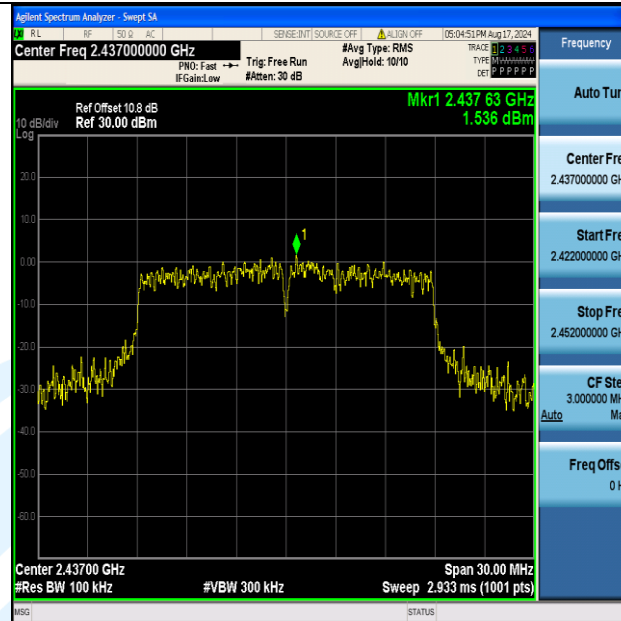
11N20MIMO-Ant2-2437-0~Reference-PASS
