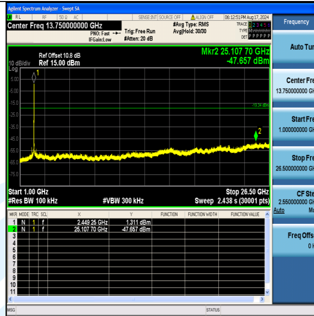
11N40MIMO-Ant2-2452-1000-26500-PASS
