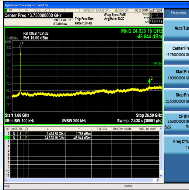
11N40MIMO-Ant2-2437-1000-26500-PASS
