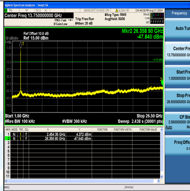
11G-Ant2-2462-1000~26500-PASS
