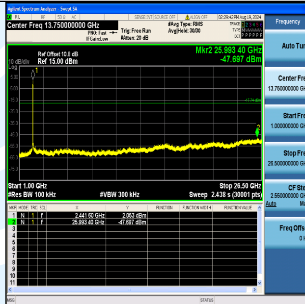
11N40MIMO-Ant1-2452-0-Reference-PASS
