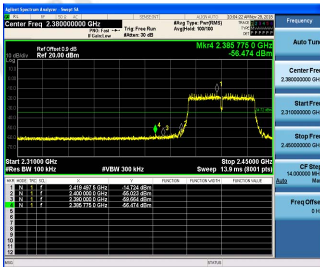
Left bandedge
