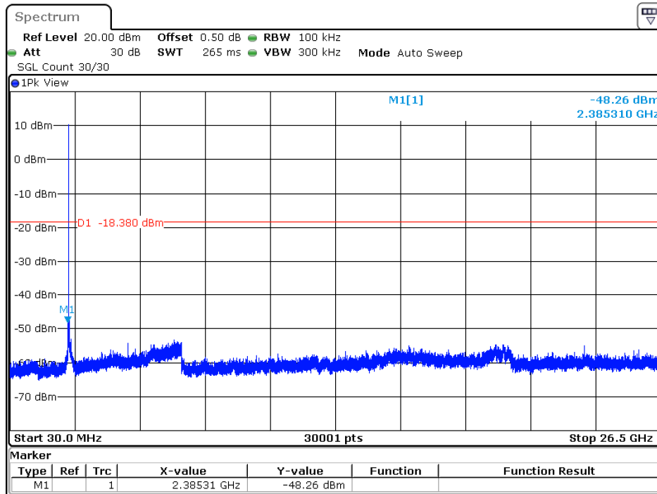
Channel 01 (2412 MHz)
