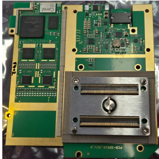
Internal photo of the product with the board
