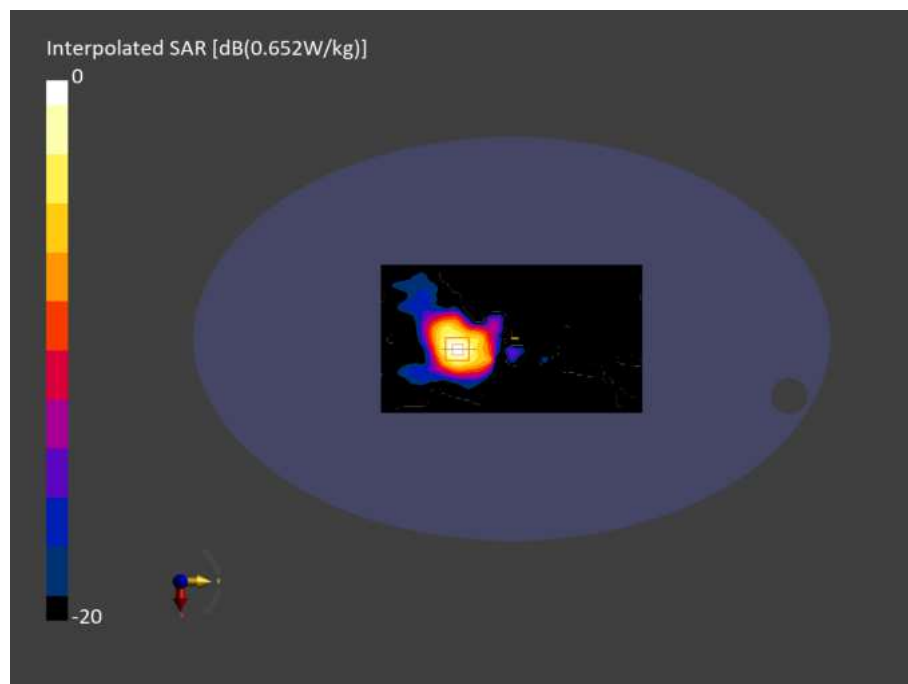
Figure C.02: Testing results for the IMAGO L with Linear Probe at 5200MHz
