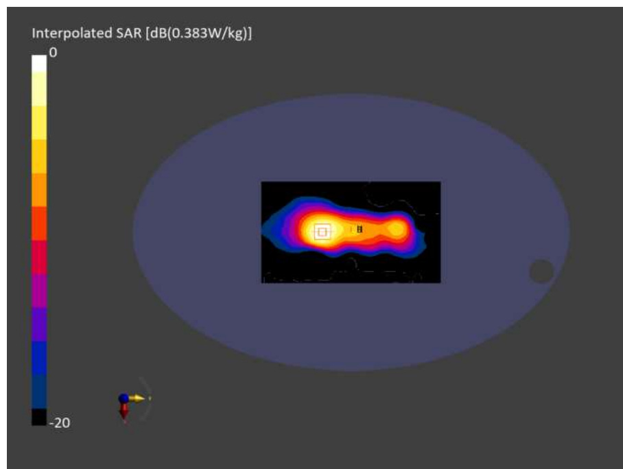
Figure C.03: Testing results for the IMAGO C with Curved Probe at 2437MHz
