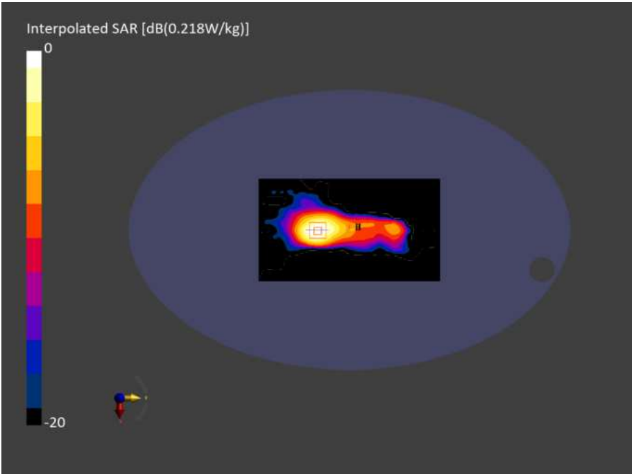
Figure C.01: Testing results for the IMAGO L with Linear Probe at 2437MHz
