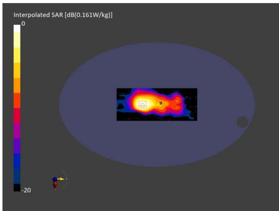
Figure C.05: Testing results for the IMAGO FLEX with Removable Probe at 2437MHz
