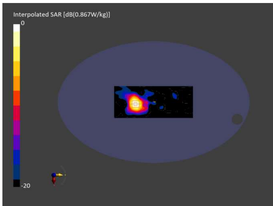
Figure C.06: Testing results for the IMAGO FLEX with Removable Probe at 5180MHz
