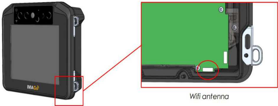
Figure 2: IMAGO FLEX (Multi) with removable Probe
