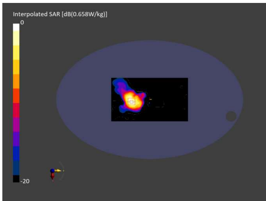
Figure C.04: Testing results for the IMAGO C with Curved Probe at 5180MHz
