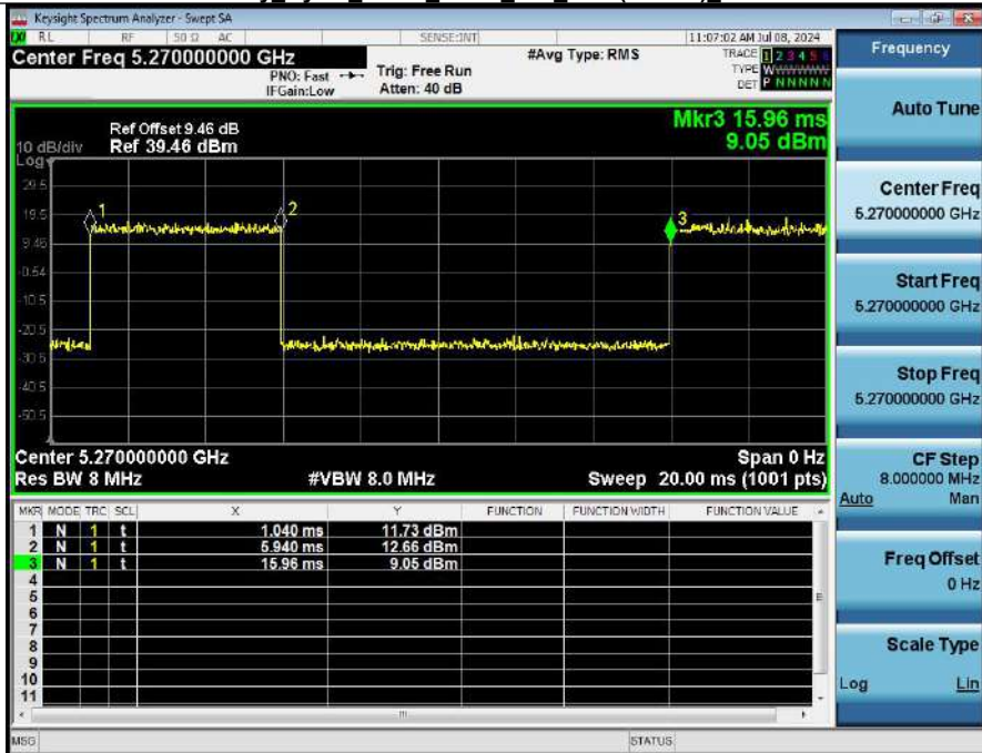
Duty_Cycle_NVNT_ANT1_802_11ac(VHT40)_5270
